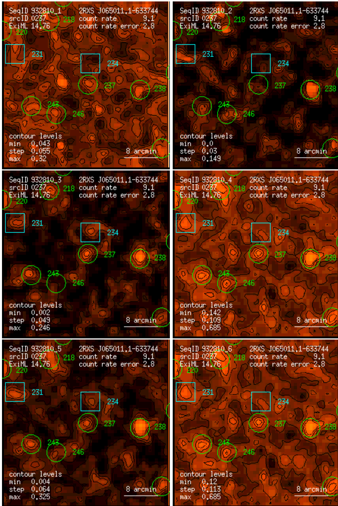
Figure 237: RASS 932810: detection 0237: band rate images, Gaussian filter: (1) PSPC channels 11 – 41, (2) 52 – 90, (3) 91 – 201, (4) 11 – 235, (5) 52 – 201, (6) 11 – 201. Broad band rates in counts/ks. Band rate contour levels in counts/ks/arcmin 2 .
