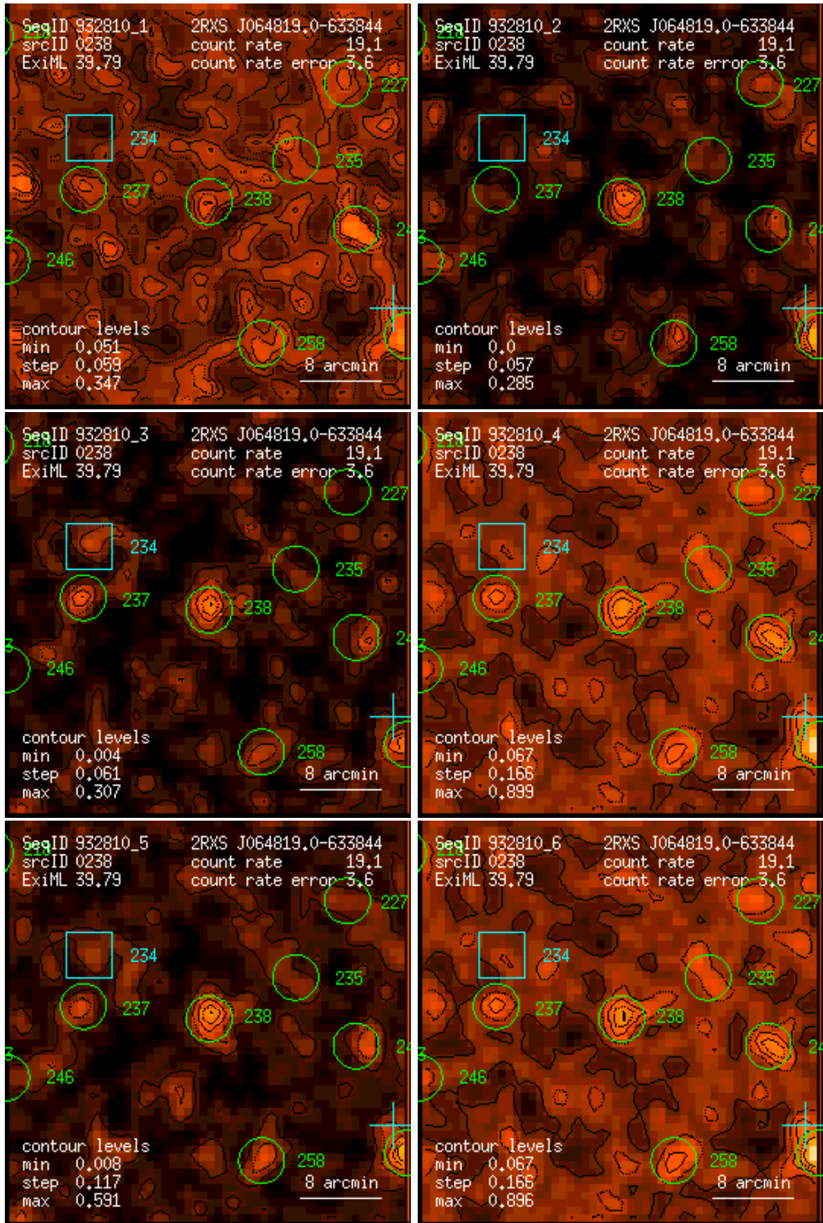
Figure 238: RASS 932810: detection 0238: band rate images, Gaussian filter: (1) PSPC channels 11 – 41, (2) 52 – 90, (3) 91 – 201, (4) 11 – 235, (5) 52 – 201, (6) 11 – 201. Broad band rates in counts/ks. Band rate contour levels in counts/ks/arcmin 2 .
