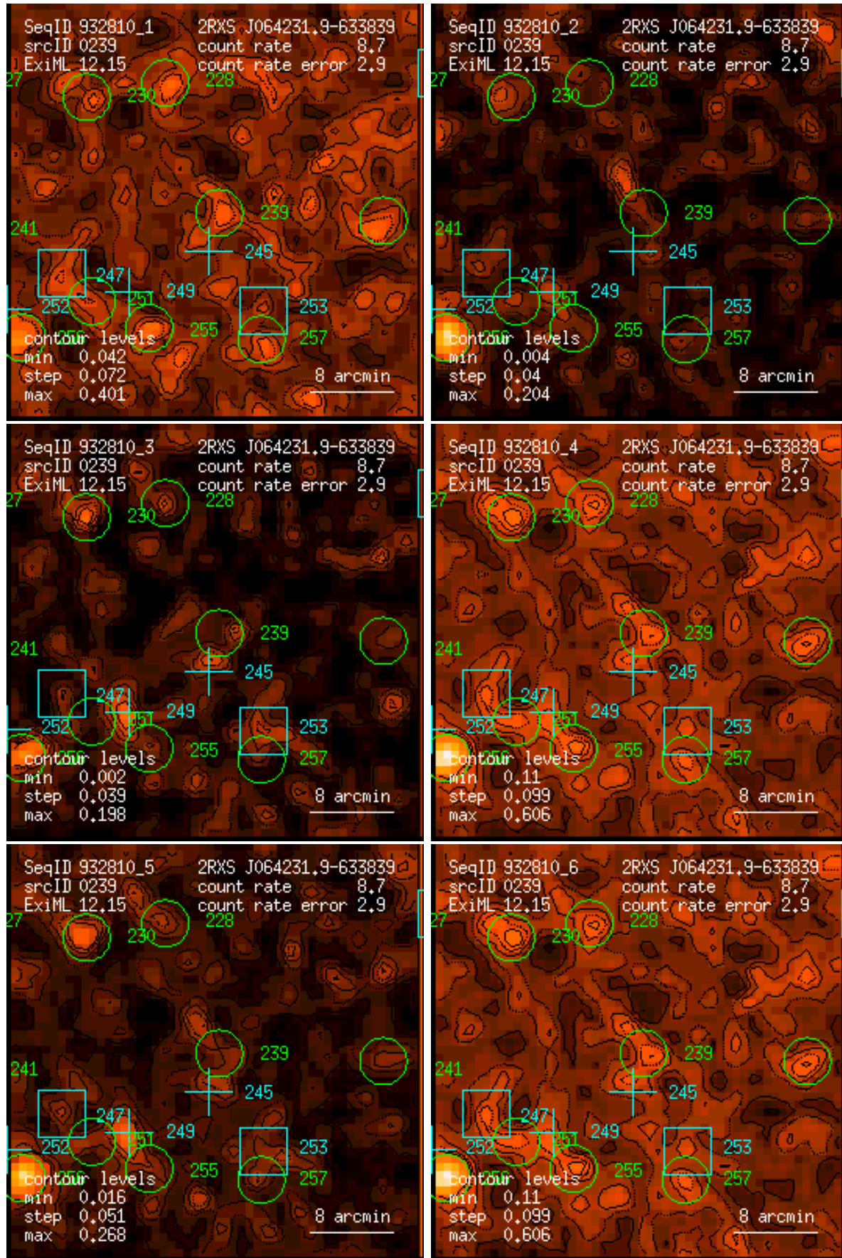
Figure 239: RASS 932810: detection 0239: band rate images, Gaussian filter: (1) PSPC channels 11 – 41, (2) 52 – 90, (3) 91 – 201, (4) 11 – 235, (5) 52 – 201, (6) 11 – 201. Broad band rates in counts/ks. Band rate contour levels in counts/ks/arcmin 2 .
