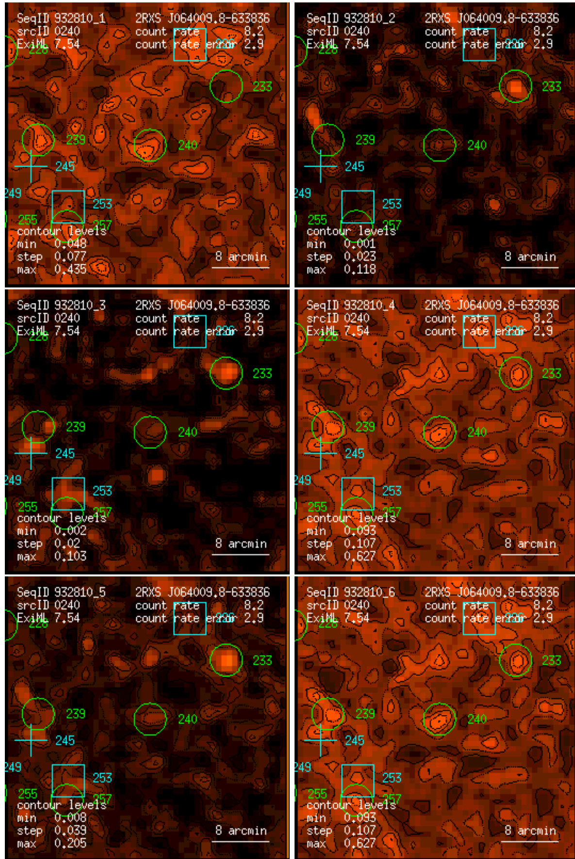
Figure 240: RASS 932810: detection 0240: band rate images, Gaussian filter: (1) PSPC channels 11 – 41, (2) 52 – 90, (3) 91 – 201, (4) 11 – 235, (5) 52 – 201, (6) 11 – 201. Broad band rates in counts/ks. Band rate contour levels in counts/ks/arcmin 2 .
