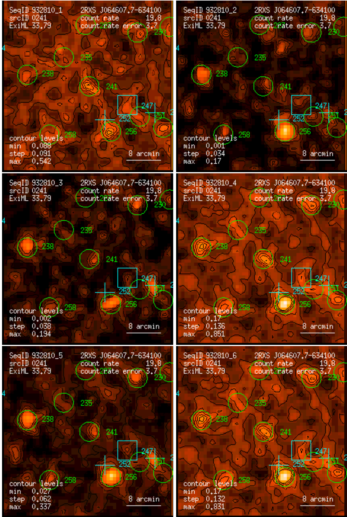
Figure 241: RASS 932810: detection 0241: band rate images, Gaussian filter: (1) PSPC channels 11 – 41, (2) 52 – 90, (3) 91 – 201, (4) 11 – 235, (5) 52 – 201, (6) 11 – 201. Broad band rates in counts/ks. Band rate contour levels in counts/ks/arcmin 2 .
