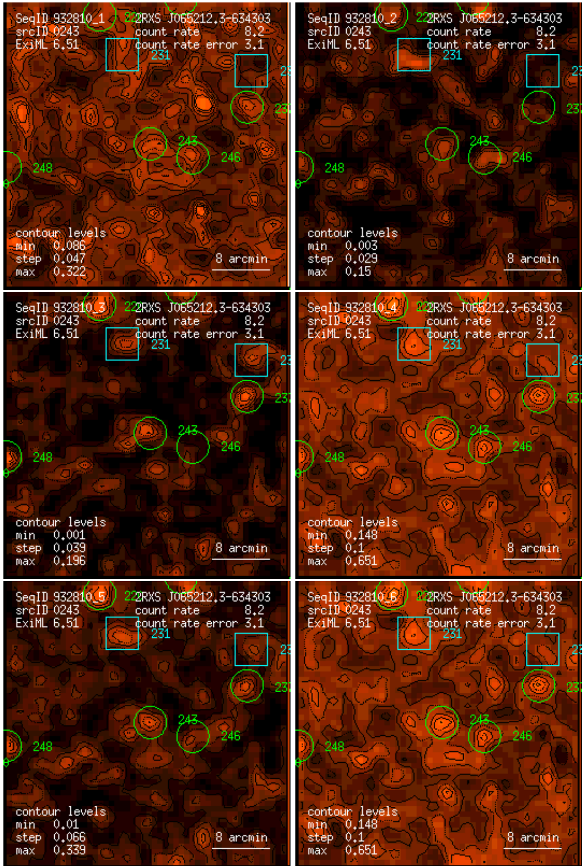
Figure 243: RASS 932810: detection 0243: band rate images, Gaussian filter: (1) PSPC channels 11 – 41, (2) 52 – 90, (3) 91 – 201, (4) 11 – 235, (5) 52 – 201, (6) 11 – 201. Broad band rates in counts/ks. Band rate contour levels in counts/ks/arcmin 2 .
