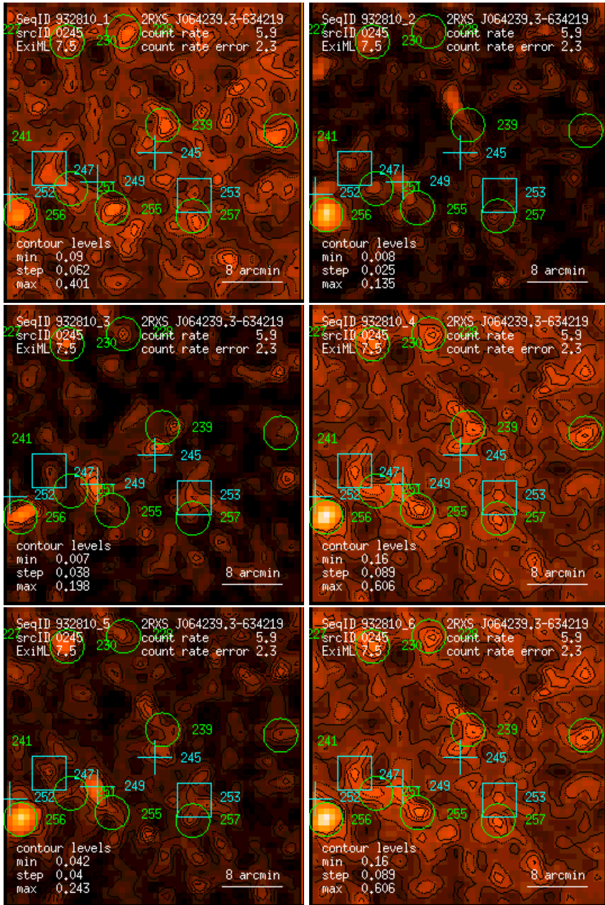
Figure 245: RASS 932810: detection 0245: band rate images, Gaussian filter: (1) PSPC channels 11 – 41, (2) 52 – 90, (3) 91 – 201, (4) 11 – 235, (5) 52 – 201, (6) 11 – 201. Broad band rates in counts/ks. Band rate contour levels in counts/ks/arcmin 2 .
