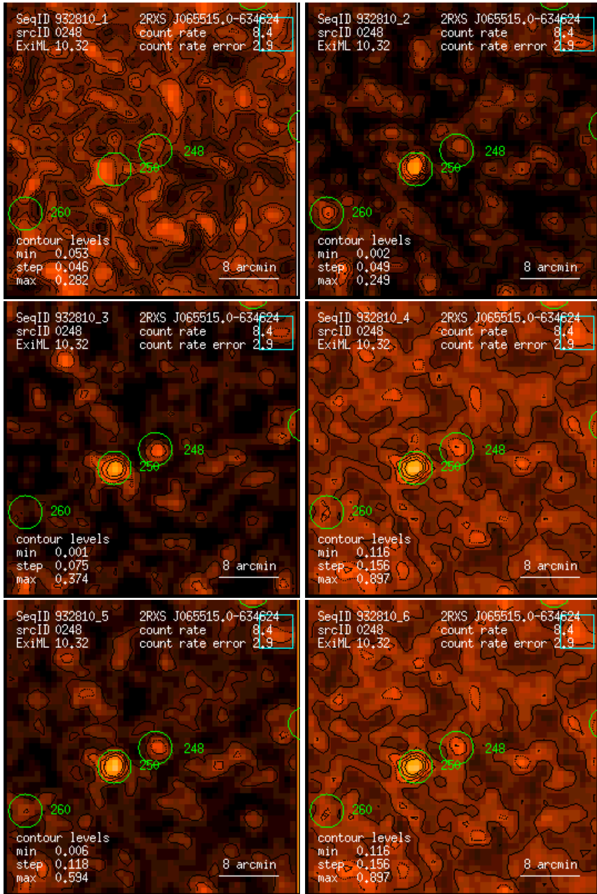
Figure 248: RASS 932810: detection 0248: band rate images, Gaussian filter: (1) PSPC channels 11 – 41, (2) 52 – 90, (3) 91 – 201, (4) 11 – 235, (5) 52 – 201, (6) 11 – 201. Broad band rates in counts/ks. Band rate contour levels in counts/ks/arcmin 2 .
