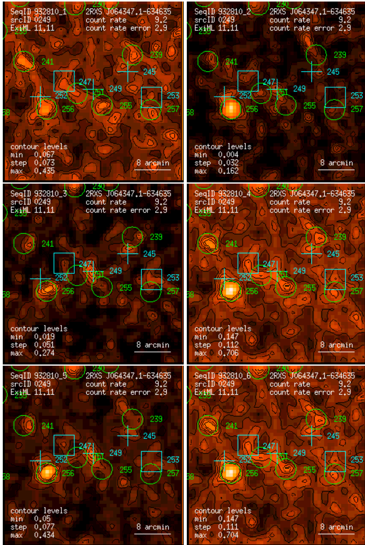
Figure 249: RASS 932810: detection 0249: band rate images, Gaussian filter: (1) PSPC channels 11 – 41, (2) 52 – 90, (3) 91 – 201, (4) 11 – 235, (5) 52 – 201, (6) 11 – 201. Broad band rates in counts/ks. Band rate contour levels in counts/ks/arcmin 2 .
