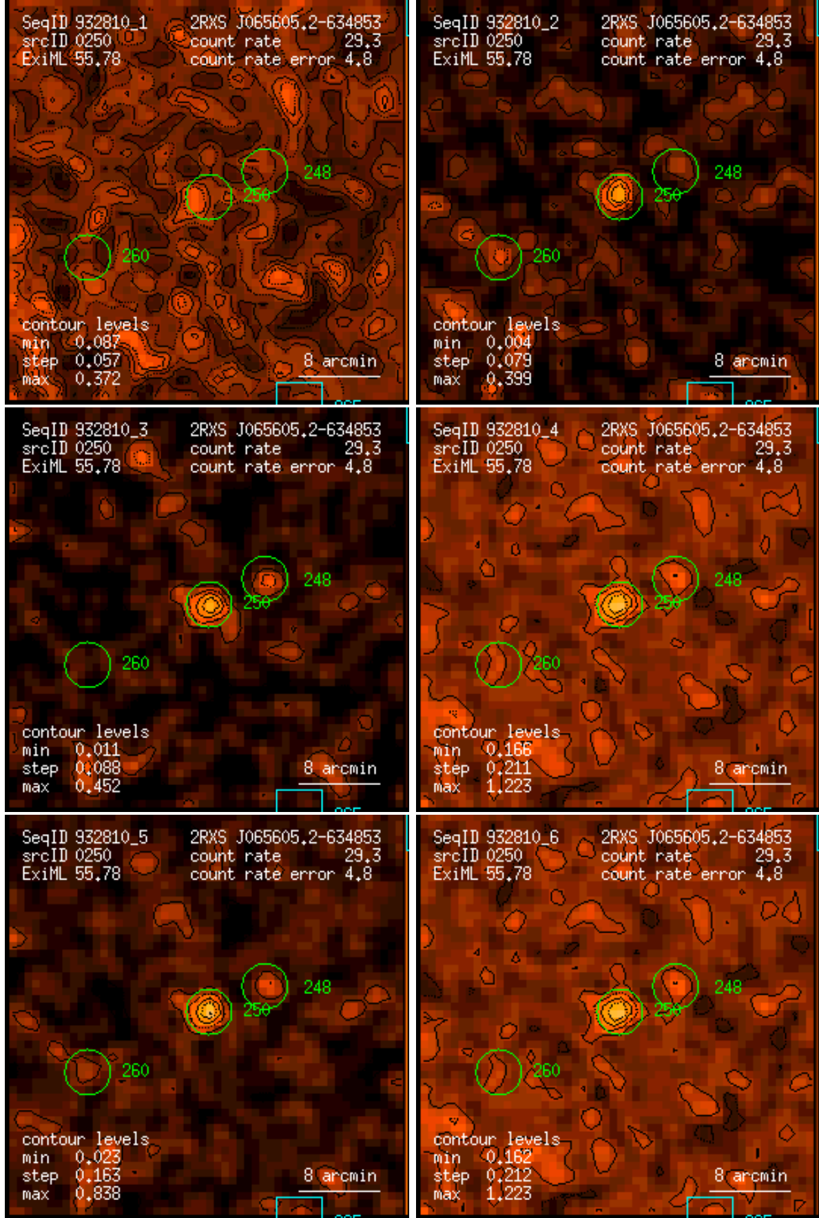
Figure 250: RASS 932810: detection 0250: band rate images, Gaussian filter: (1) PSPC channels 11 – 41, (2) 52 – 90, (3) 91 – 201, (4) 11 – 235, (5) 52 – 201, (6) 11 – 201. Broad band rates in counts/ks. Band rate contour levels in counts/ks/arcmin 2 .
