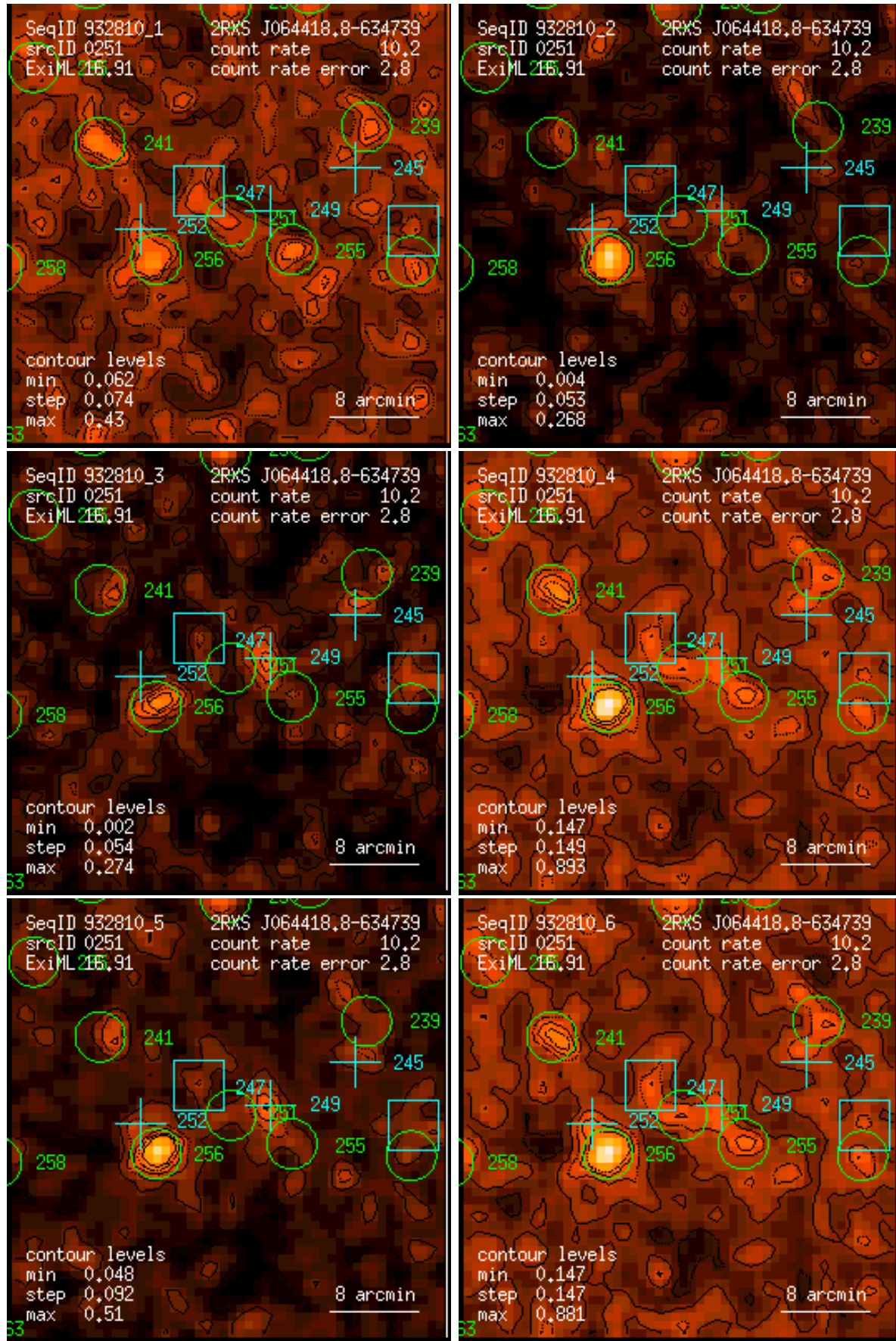
Figure 251: RASS 932810: detection 0251: band rate images, Gaussian filter: (1) PSPC channels 11 – 41, (2) 52 – 90, (3) 91 – 201, (4) 11 – 235, (5) 52 – 201, (6) 11 – 201. Broad band rates in counts/ks. Band rate contour levels in counts/ks/arcmin 2 .
