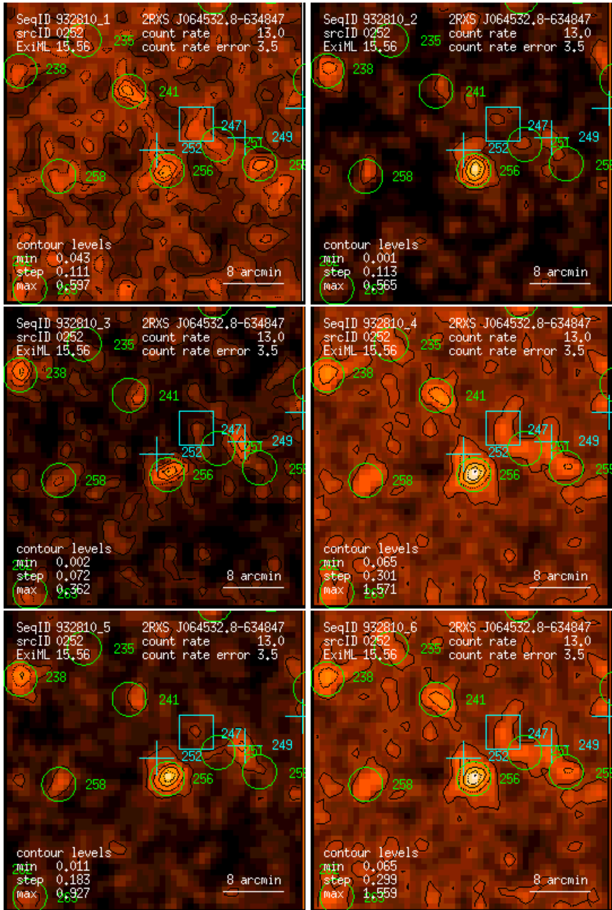
Figure 252: RASS 932810: detection 0252: band rate images, Gaussian filter: (1) PSPC channels 11 – 41, (2) 52 – 90, (3) 91 – 201, (4) 11 – 235, (5) 52 – 201, (6) 11 – 201. Broad band rates in counts/ks. Band rate contour levels in counts/ks/arcmin 2 .
