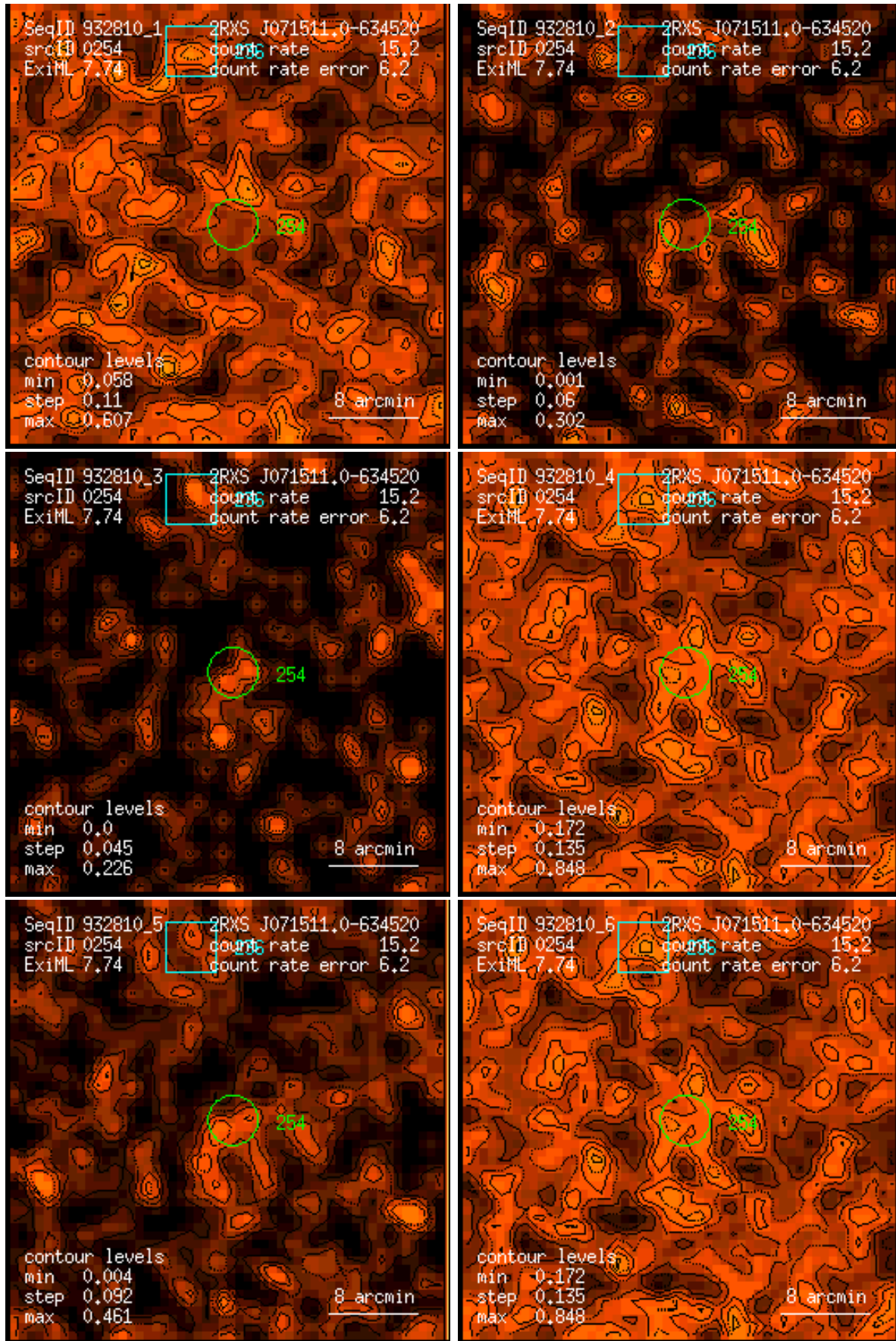
Figure 254: RASS 932810: detection 0254: band rate images, Gaussian filter: (1) PSPC channels 11 – 41, (2) 52 – 90, (3) 91 – 201, (4) 11 – 235, (5) 52 – 201, (6) 11 – 201. Broad band rates in counts/ks. Band rate contour levels in counts/ks/arcmin 2 .
