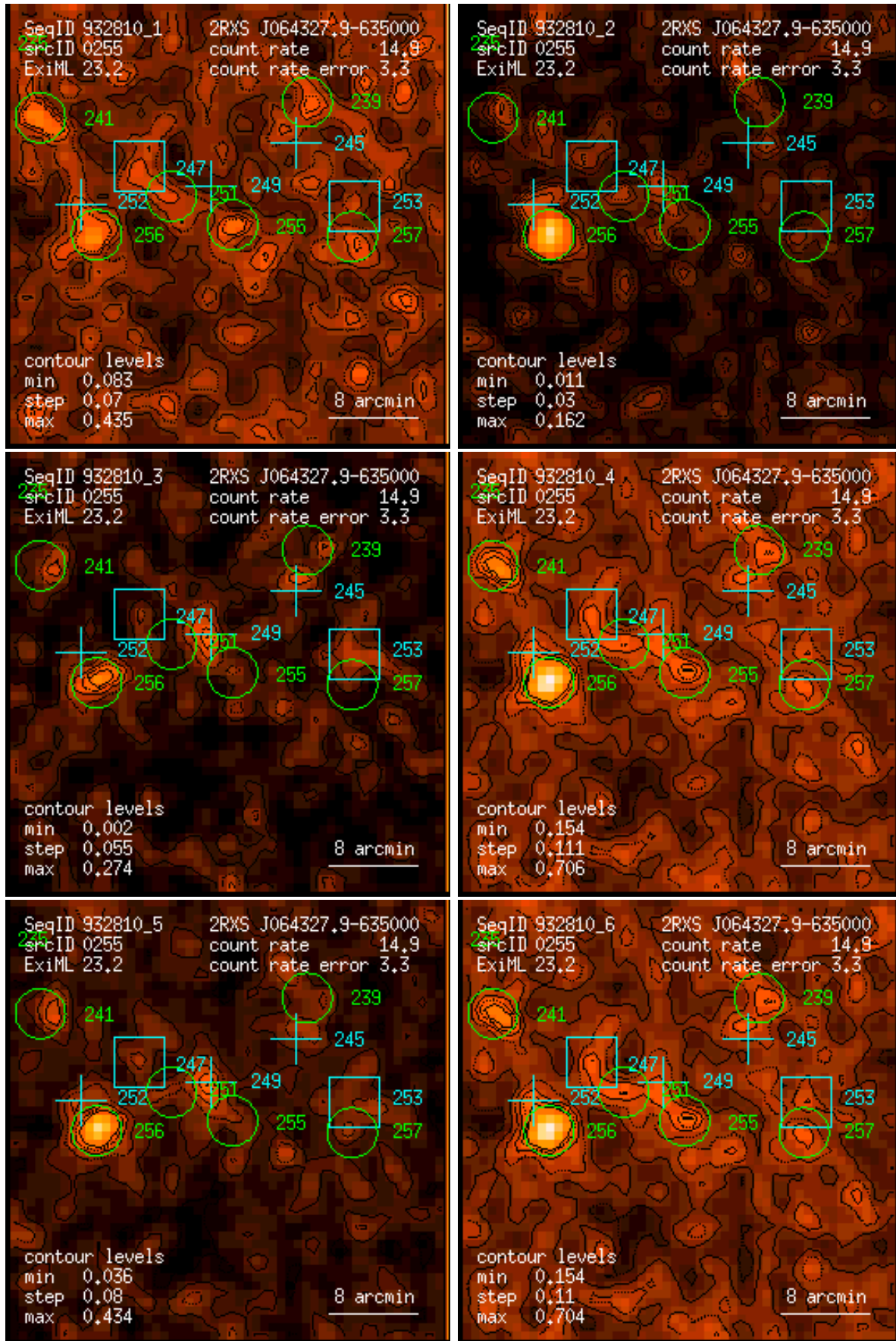
Figure 255: RASS 932810: detection 0255: band rate images, Gaussian filter: (1) PSPC channels 11 – 41, (2) 52 – 90, (3) 91 – 201, (4) 11 – 235, (5) 52 – 201, (6) 11 – 201. Broad band rates in counts/ks. Band rate contour levels in counts/ks/arcmin 2 .
