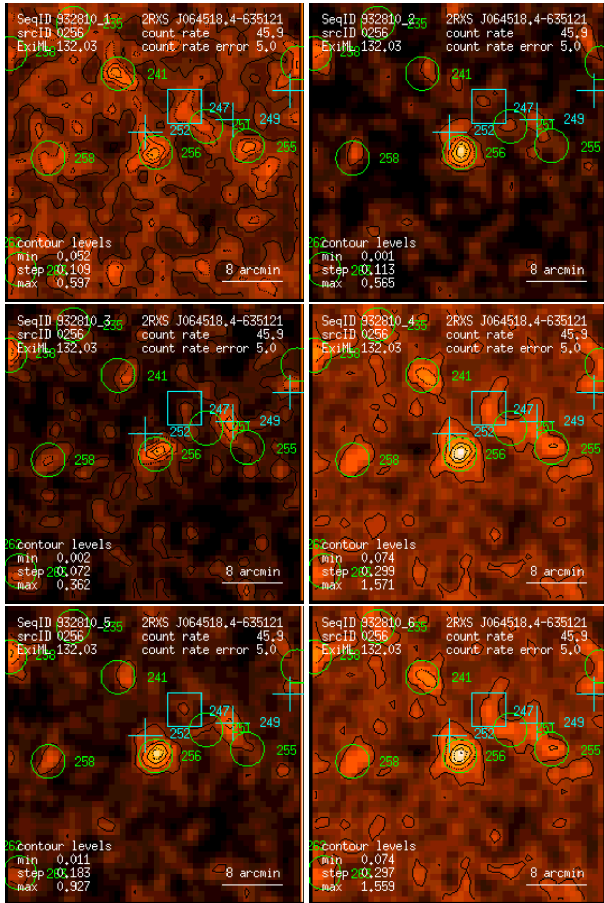
Figure 256: RASS 932810: detection 0256: band rate images, Gaussian filter: (1) PSPC channels 11 – 41, (2) 52 – 90, (3) 91 – 201, (4) 11 – 235, (5) 52 – 201, (6) 11 – 201. Broad band rates in counts/ks. Band rate contour levels in counts/ks/arcmin 2 .
