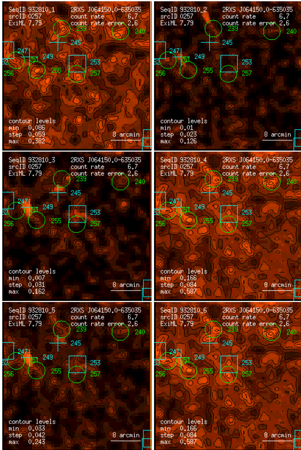
Figure 257: RASS 932810: detection 0257: band rate images, Gaussian filter: (1) PSPC channels 11 – 41, (2) 52 – 90, (3) 91 – 201, (4) 11 – 235, (5) 52 – 201, (6) 11 – 201. Broad band rates in counts/ks. Band rate contour levels in counts/ks/arcmin 2 .
