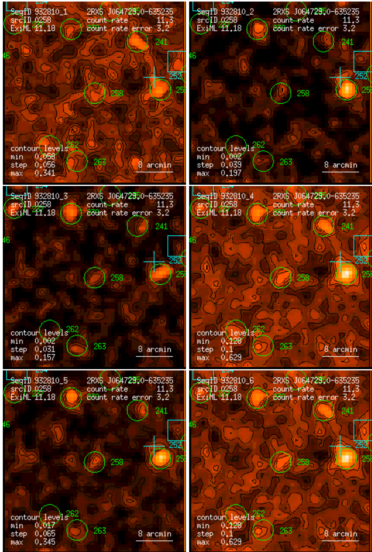
Figure 258: RASS 932810: detection 0258: band rate images, Gaussian filter: (1) PSPC channels 11 – 41, (2) 52 – 90, (3) 91 – 201, (4) 11 – 235, (5) 52 – 201, (6) 11 – 201. Broad band rates in counts/ks. Band rate contour levels in counts/ks/arcmin 2 .
