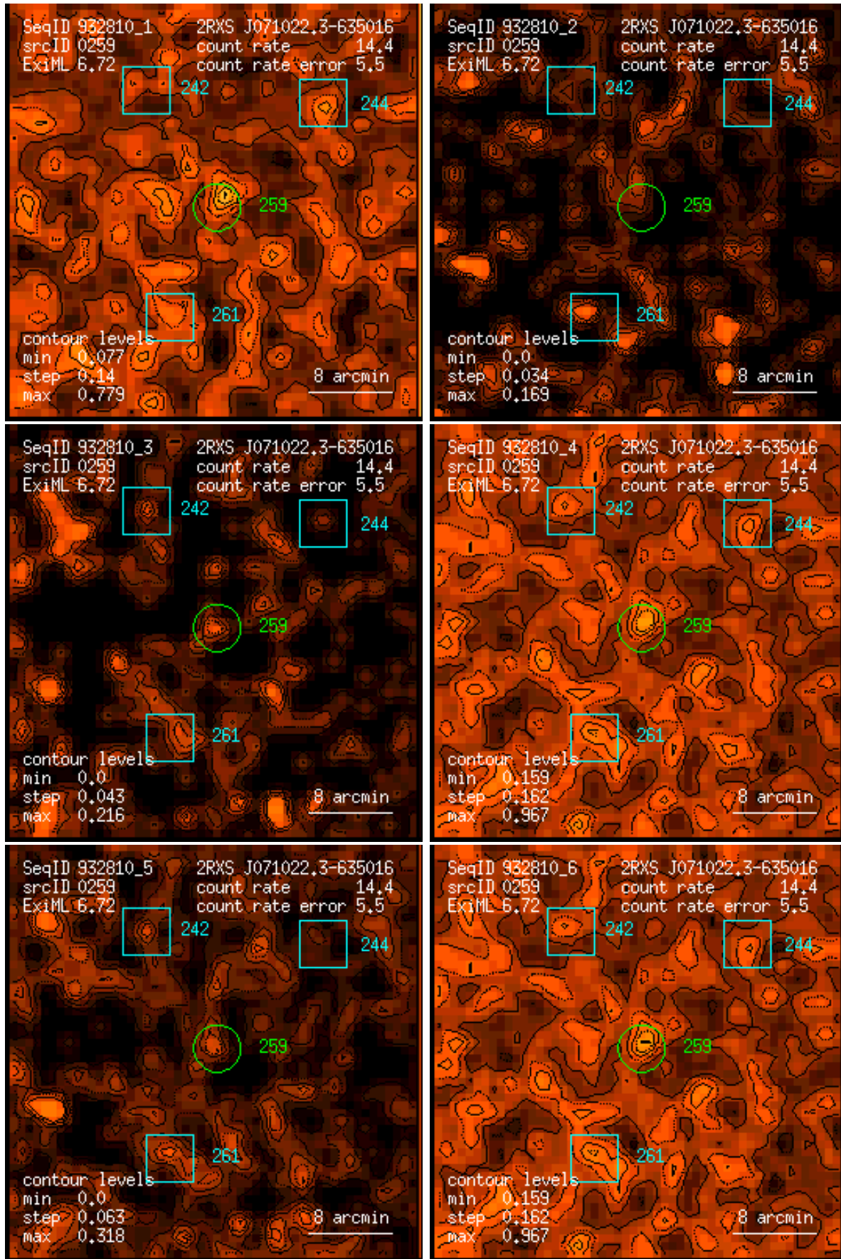
Figure 259: RASS 932810: detection 0259: band rate images, Gaussian filter: (1) PSPC channels 11 – 41, (2) 52 – 90, (3) 91 – 201, (4) 11 – 235, (5) 52 – 201, (6) 11 – 201. Broad band rates in counts/ks. Band rate contour levels in counts/ks/arcmin 2 .
