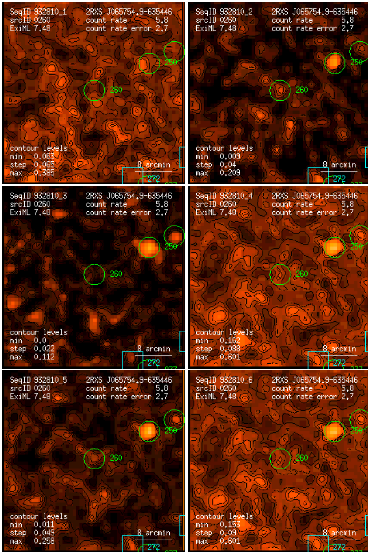
Figure 260: RASS 932810: detection 0260: band rate images, Gaussian filter: (1) PSPC channels 11 – 41, (2) 52 – 90, (3) 91 – 201, (4) 11 – 235, (5) 52 – 201, (6) 11 – 201. Broad band rates in counts/ks. Band rate contour levels in counts/ks/arcmin 2 .
