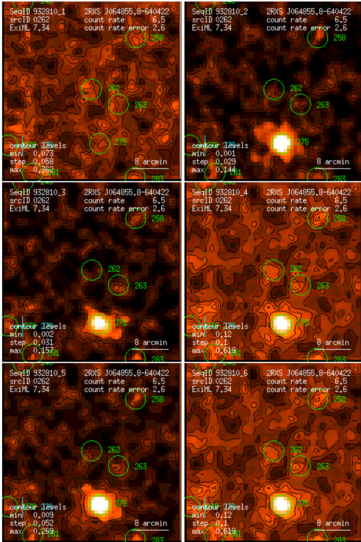
Figure 262: RASS 932810: detection 0262: band rate images, Gaussian filter: (1) PSPC channels 11 – 41, (2) 52 – 90, (3) 91 – 201, (4) 11 – 235, (5) 52 – 201, (6) 11 – 201. Broad band rates in counts/ks. Band rate contour levels in counts/ks/arcmin 2 .
