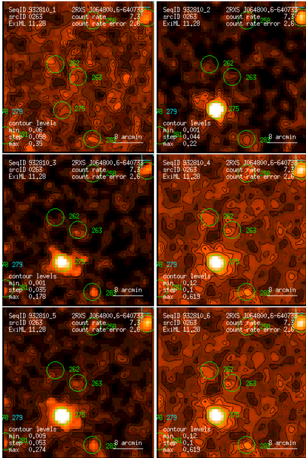
Figure 263: RASS 932810: detection 0263: band rate images, Gaussian filter: (1) PSPC channels 11 – 41, (2) 52 – 90, (3) 91 – 201, (4) 11 – 235, (5) 52 – 201, (6) 11 – 201. Broad band rates in counts/ks. Band rate contour levels in counts/ks/arcmin 2 .
