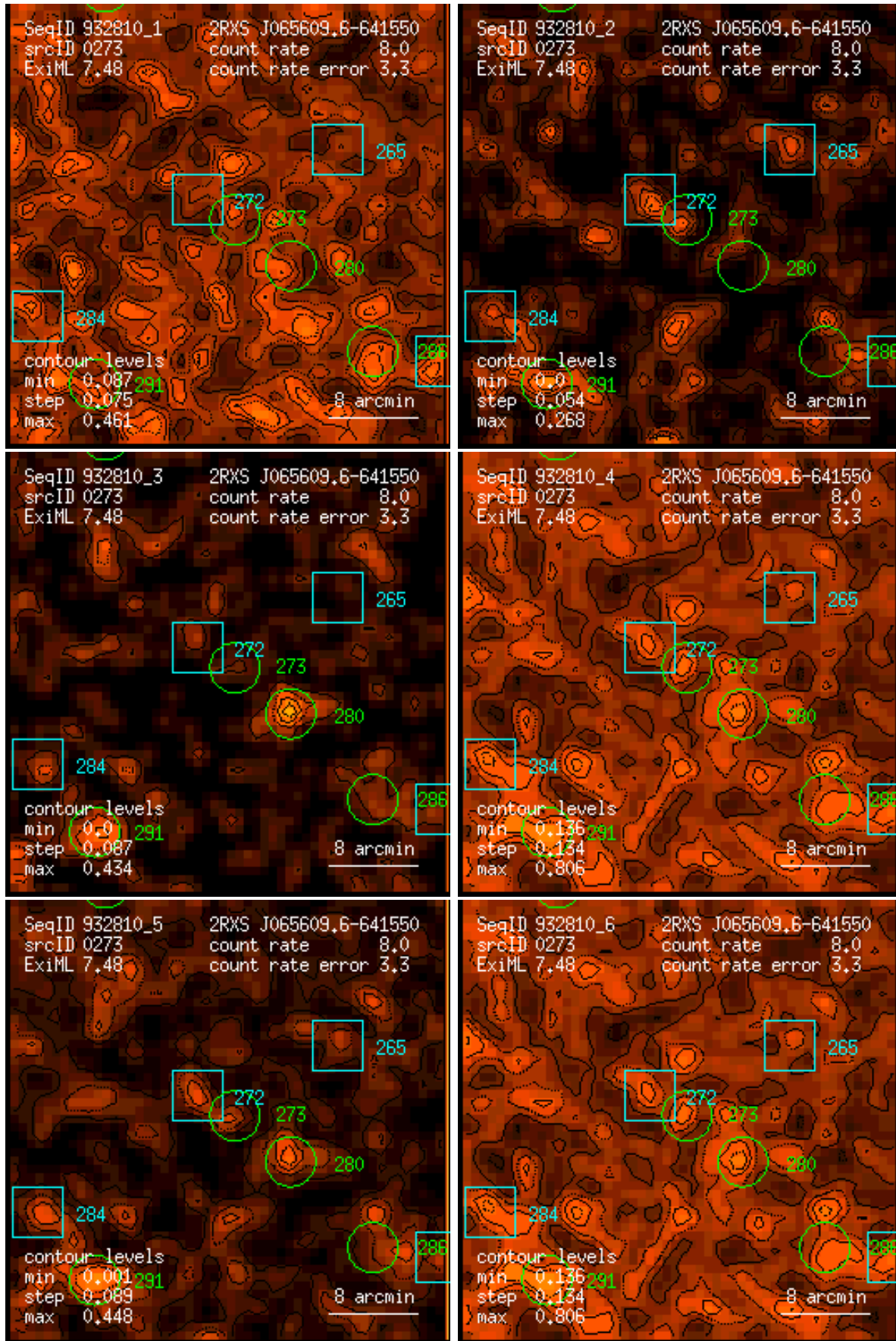
Figure 273: RASS 932810: detection 0273: band rate images, Gaussian filter: (1) PSPC channels 11 – 41, (2) 52 – 90, (3) 91 – 201, (4) 11 – 235, (5) 52 – 201, (6) 11 – 201. Broad band rates in counts/ks. Band rate contour levels in counts/ks/arcmin 2 .
