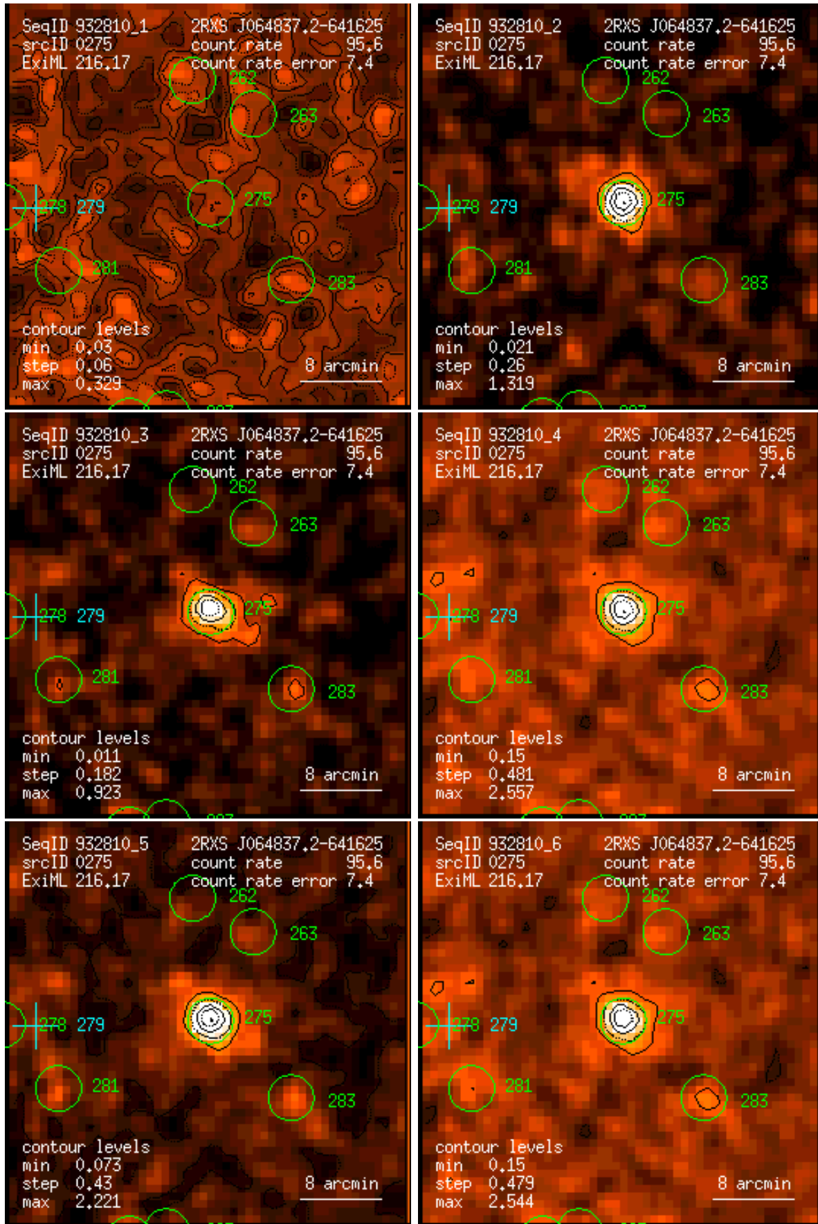
Figure 275: RASS 932810: detection 0275: band rate images, Gaussian filter: (1) PSPC channels 11 – 41, (2) 52 – 90, (3) 91 – 201, (4) 11 – 235, (5) 52 – 201, (6) 11 – 201. Broad band rates in counts/ks. Band rate contour levels in counts/ks/arcmin 2 .
