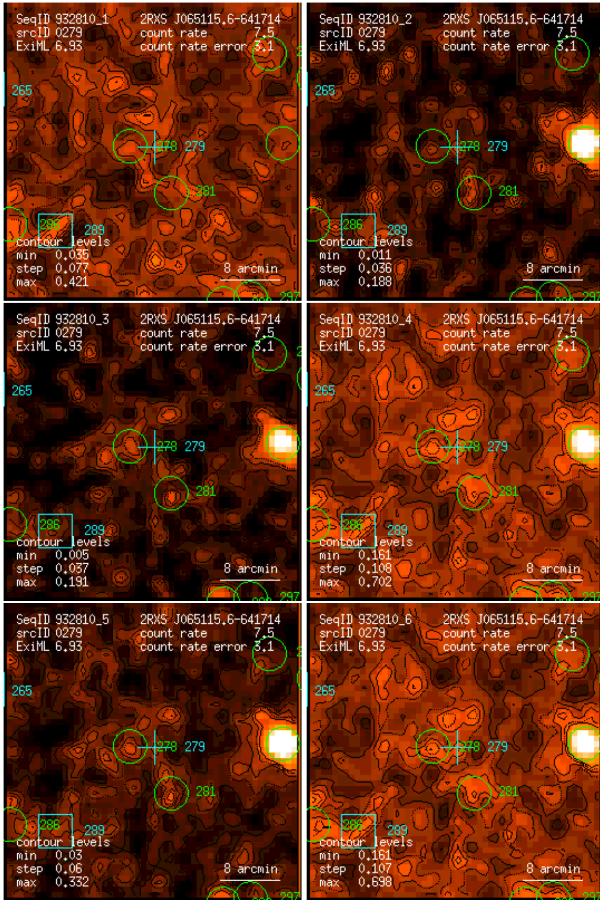
Figure 279: RASS 932810: detection 0279: band rate images, Gaussian filter: (1) PSPC channels 11 – 41, (2) 52 – 90, (3) 91 – 201, (4) 11 – 235, (5) 52 – 201, (6) 11 – 201. Broad band rates in counts/ks. Band rate contour levels in counts/ks/arcmin 2 .
