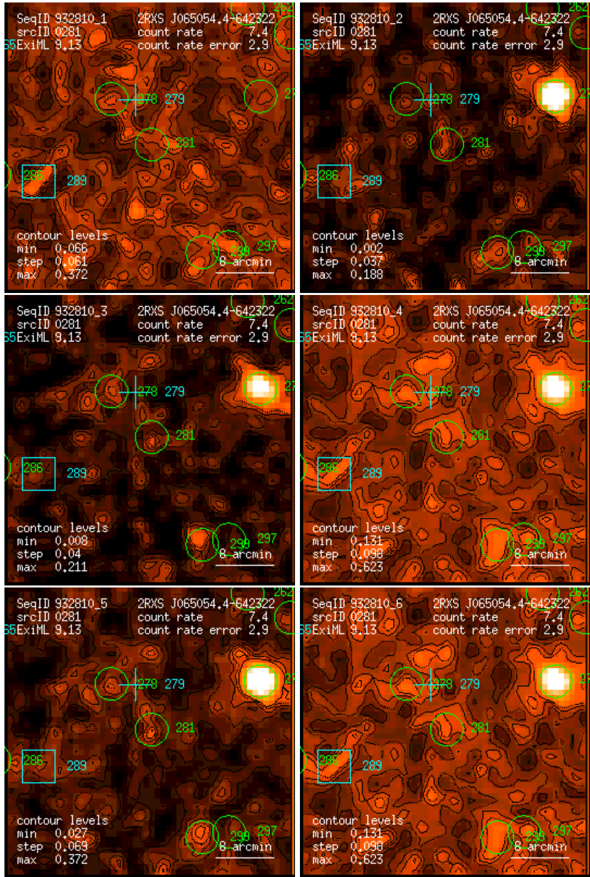
Figure 281: RASS 932810: detection 0281: band rate images, Gaussian filter: (1) PSPC channels 11 – 41, (2) 52 – 90, (3) 91 – 201, (4) 11 – 235, (5) 52 – 201, (6) 11 – 201. Broad band rates in counts/ks. Band rate contour levels in counts/ks/arcmin 2 .
