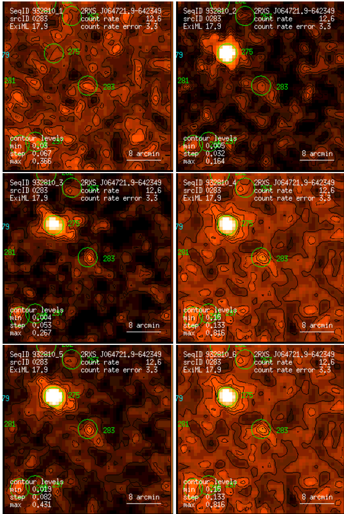
Figure 283: RASS 932810: detection 0283: band rate images, Gaussian filter: (1) PSPC channels 11 – 41, (2) 52 – 90, (3) 91 – 201, (4) 11 – 235, (5) 52 – 201, (6) 11 – 201. Broad band rates in counts/ks. Band rate contour levels in counts/ks/arcmin 2 .
