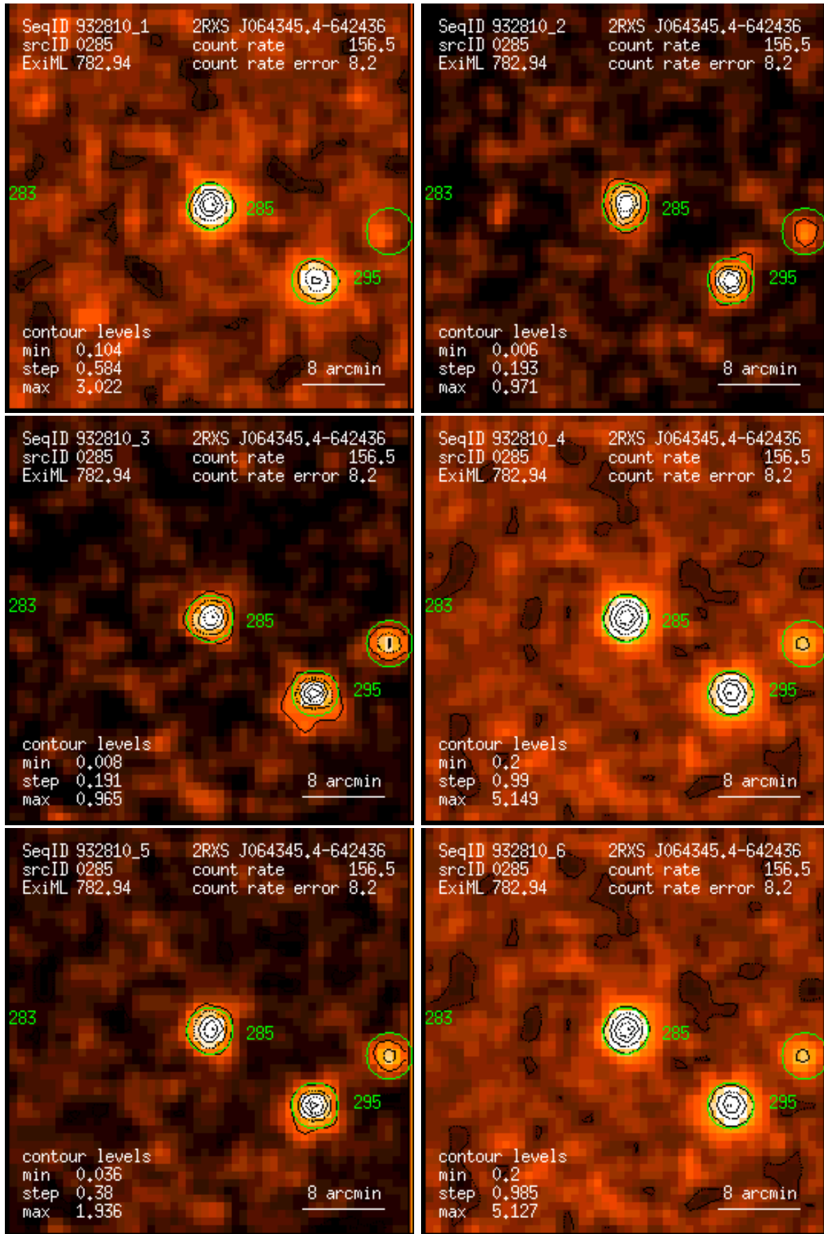
Figure 285: RASS 932810: detection 0285: band rate images, Gaussian filter: (1) PSPC channels 11 – 41, (2) 52 – 90, (3) 91 – 201, (4) 11 – 235, (5) 52 – 201, (6) 11 – 201. Broad band rates in counts/ks. Band rate contour levels in counts/ks/arcmin 2 .
