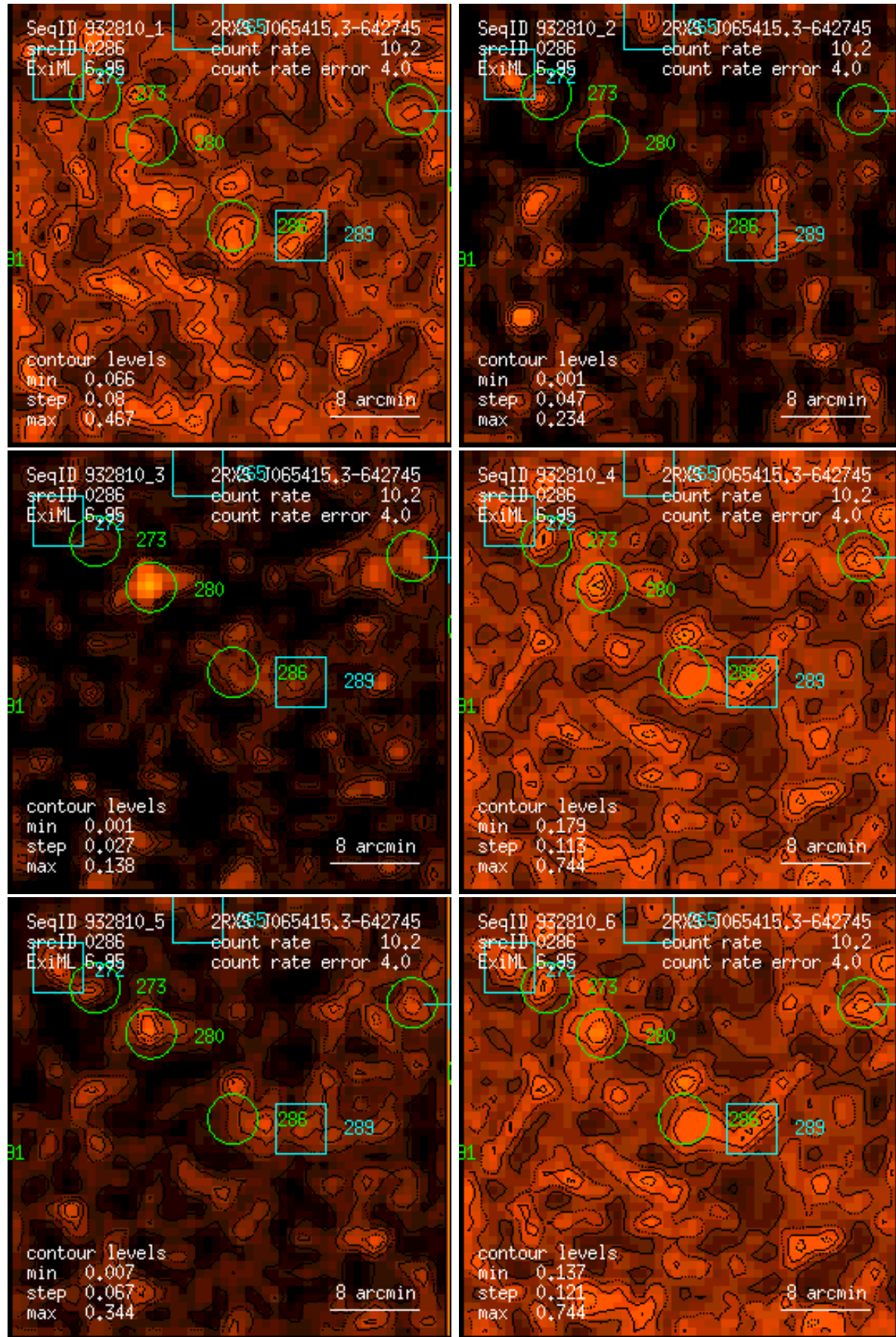
Figure 286: RASS 932810: detection 0286: band rate images, Gaussian filter: (1) PSPC channels 11 – 41, (2) 52 – 90, (3) 91 – 201, (4) 11 – 235, (5) 52 – 201, (6) 11 – 201. Broad band rates in counts/ks. Band rate contour levels in counts/ks/arcmin 2 .
