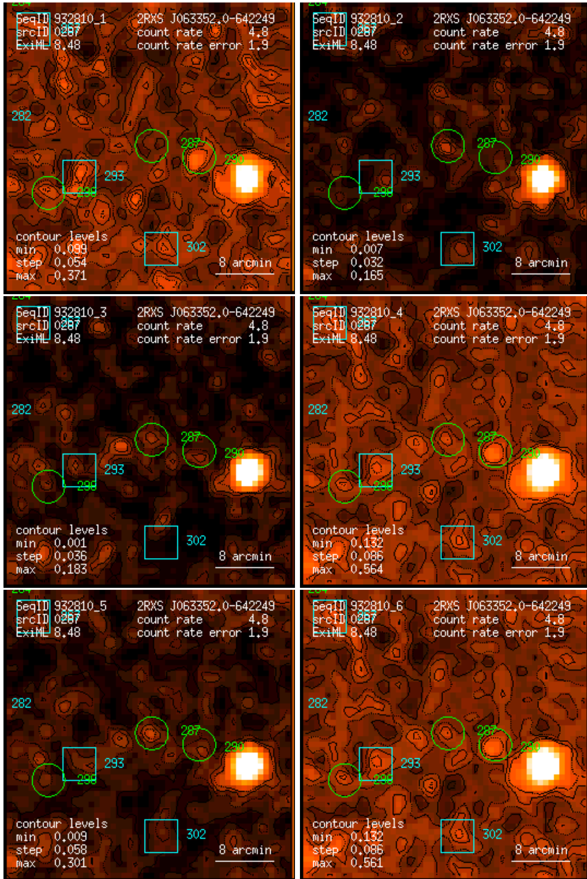
Figure 287: RASS 932810: detection 0287: band rate images, Gaussian filter: (1) PSPC channels 11 – 41, (2) 52 – 90, (3) 91 – 201, (4) 11 – 235, (5) 52 – 201, (6) 11 – 201. Broad band rates in counts/ks. Band rate contour levels in counts/ks/arcmin 2 .
