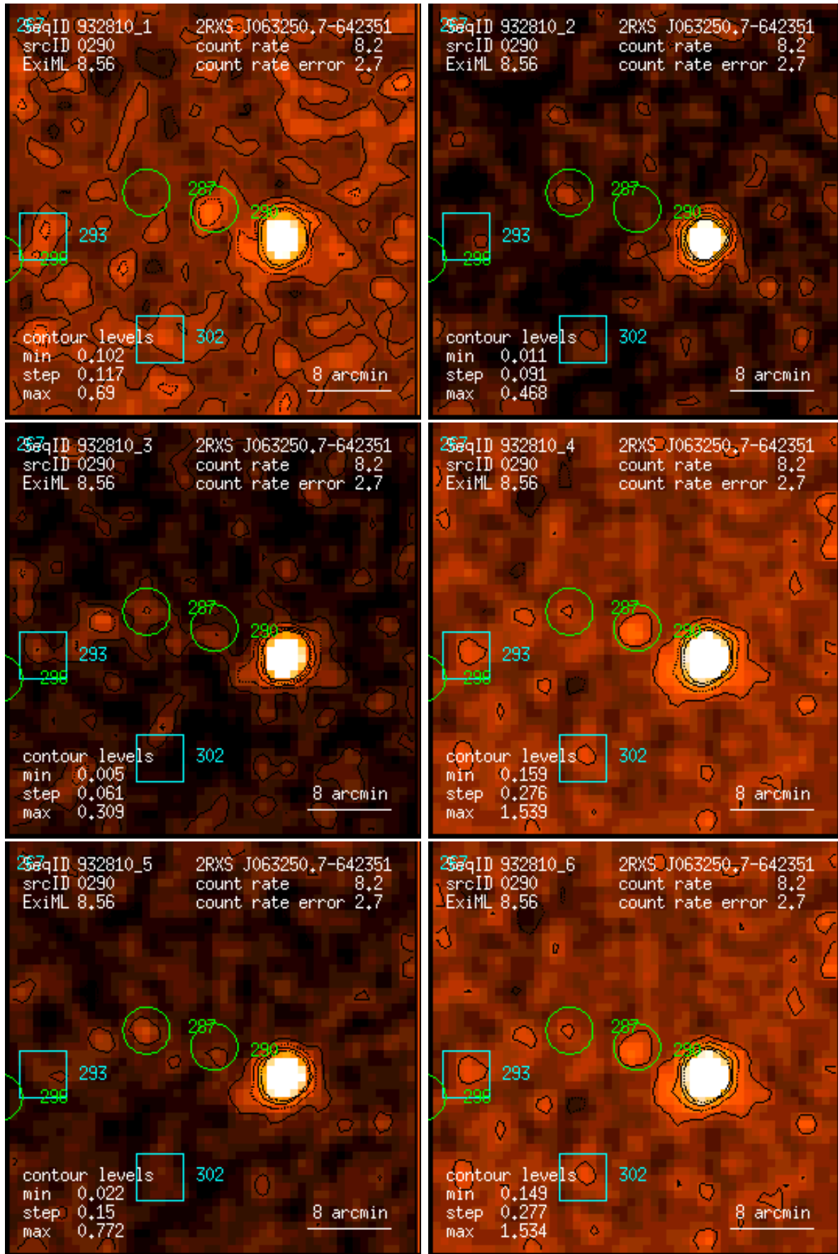
Figure 290: RASS 932810: detection 0290: band rate images, Gaussian filter: (1) PSPC channels 11 – 41, (2) 52 – 90, (3) 91 – 201, (4) 11 – 235, (5) 52 – 201, (6) 11 – 201. Broad band rates in counts/ks. Band rate contour levels in counts/ks/arcmin 2 .
