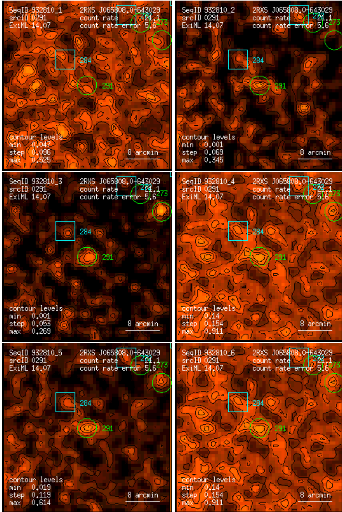
Figure 291: RASS 932810: detection 0291: band rate images, Gaussian filter: (1) PSPC channels 11 – 41, (2) 52 – 90, (3) 91 – 201, (4) 11 – 235, (5) 52 – 201, (6) 11 – 201. Broad band rates in counts/ks. Band rate contour levels in counts/ks/arcmin 2 .
