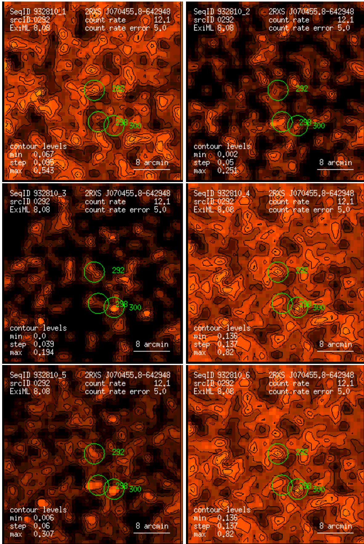
Figure 292: RASS 932810: detection 0292: band rate images, Gaussian filter: (1) PSPC channels 11 – 41, (2) 52 – 90, (3) 91 – 201, (4) 11 – 235, (5) 52 – 201, (6) 11 – 201. Broad band rates in counts/ks. Band rate contour levels in counts/ks/arcmin 2 .
