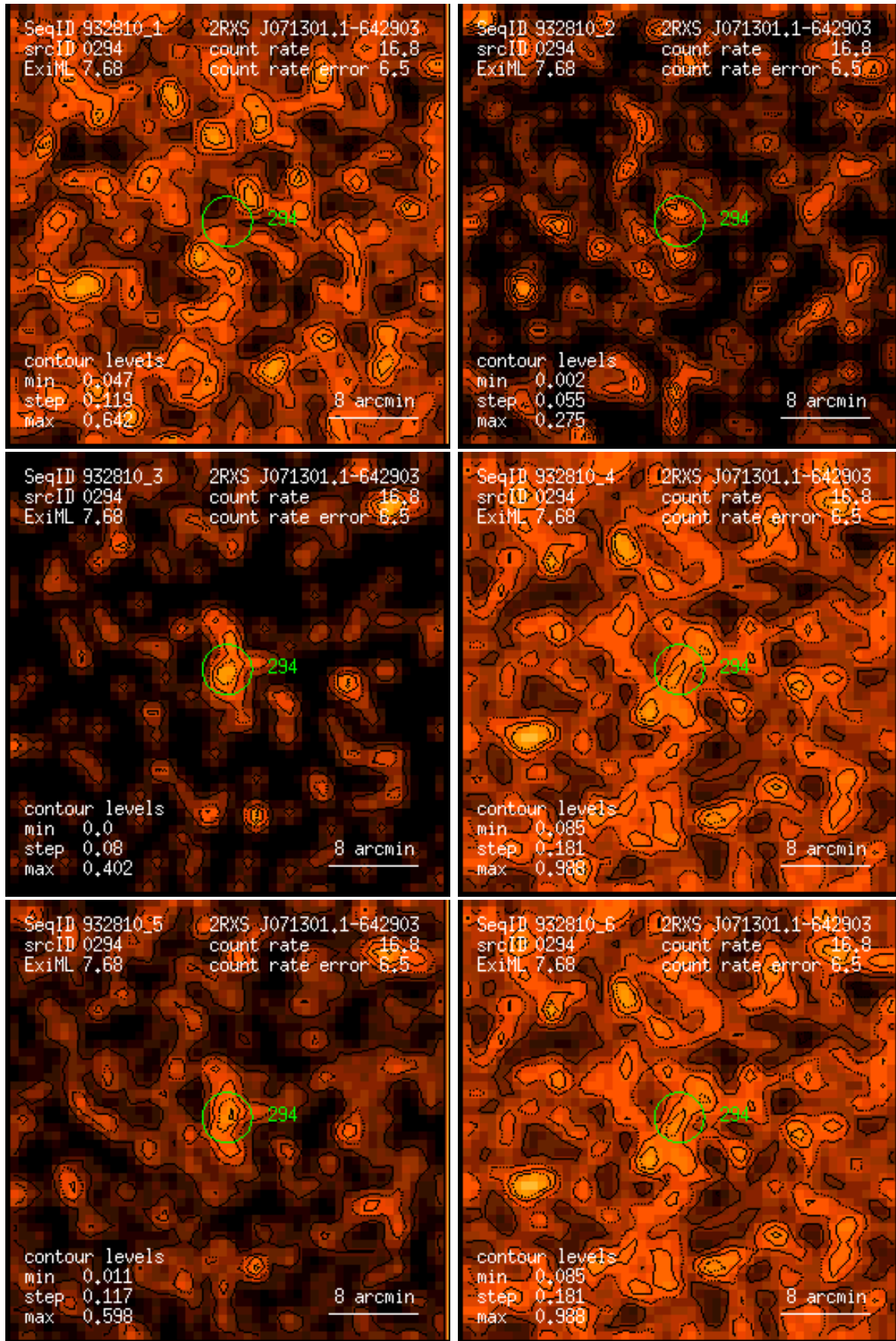
Figure 294: RASS 932810: detection 0294: band rate images, Gaussian filter: (1) PSPC channels 11 – 41, (2) 52 – 90, (3) 91 – 201, (4) 11 – 235, (5) 52 – 201, (6) 11 – 201. Broad band rates in counts/ks. Band rate contour levels in counts/ks/arcmin 2 .
