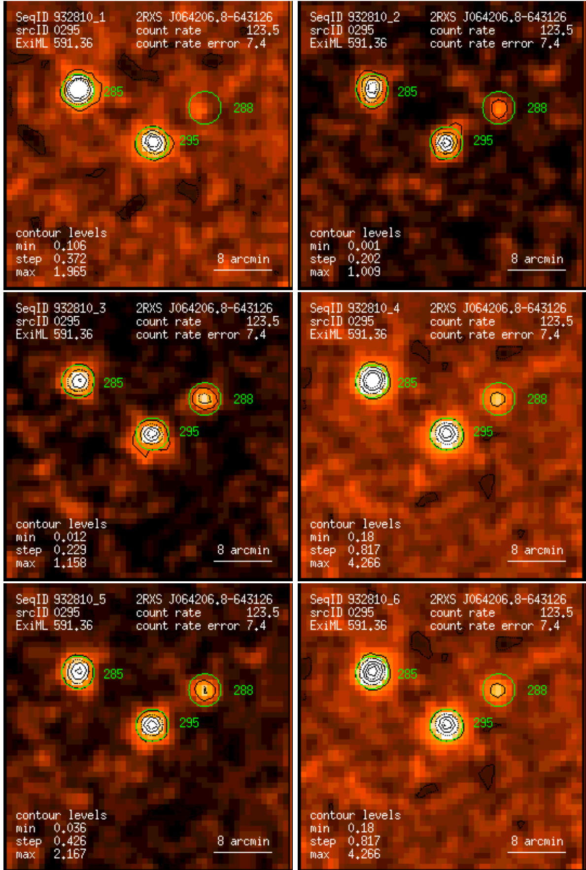
Figure 295: RASS 932810: detection 0295: band rate images, Gaussian filter: (1) PSPC channels 11 – 41, (2) 52 – 90, (3) 91 – 201, (4) 11 – 235, (5) 52 – 201, (6) 11 – 201. Broad band rates in counts/ks. Band rate contour levels in counts/ks/arcmin 2 .
