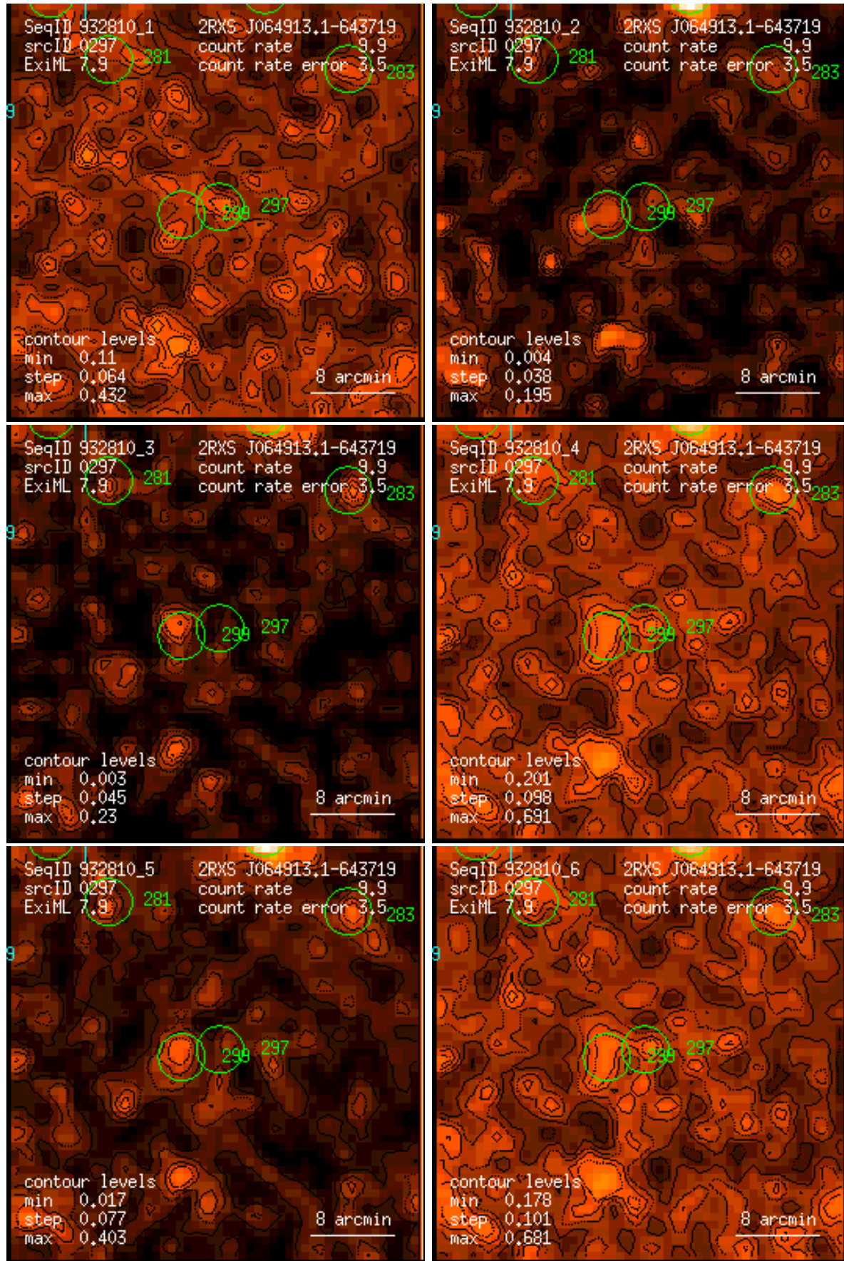
Figure 297: RASS 932810: detection 0297: band rate images, Gaussian filter: (1) PSPC channels 11 – 41, (2) 52 – 90, (3) 91 – 201, (4) 11 – 235, (5) 52 – 201, (6) 11 – 201. Broad band rates in counts/ks. Band rate contour levels in counts/ks/arcmin 2 .
