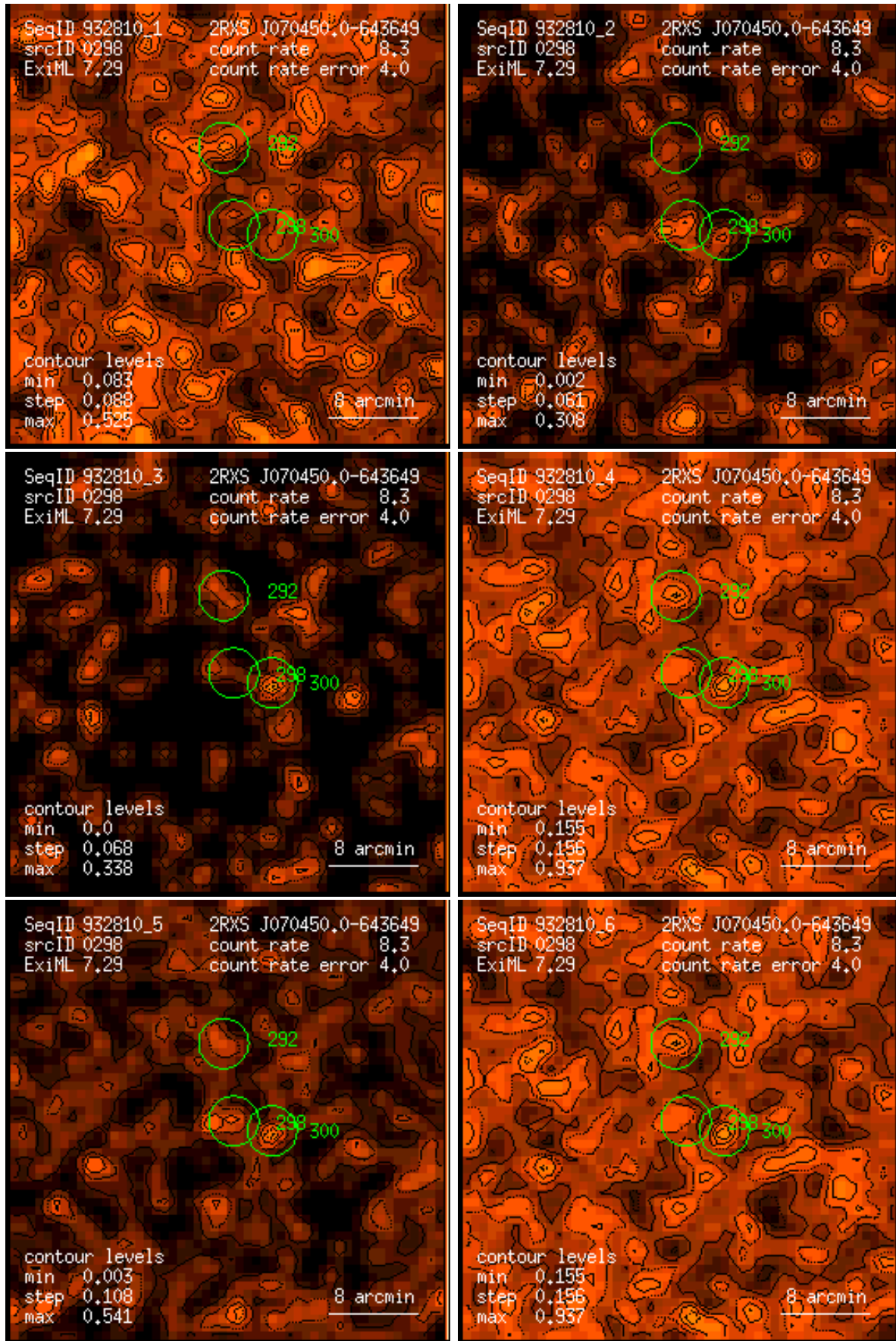
Figure 298: RASS 932810: detection 0298: band rate images, Gaussian filter: (1) PSPC channels 11 – 41, (2) 52 – 90, (3) 91 – 201, (4) 11 – 235, (5) 52 – 201, (6) 11 – 201. Broad band rates in counts/ks. Band rate contour levels in counts/ks/arcmin 2 .
