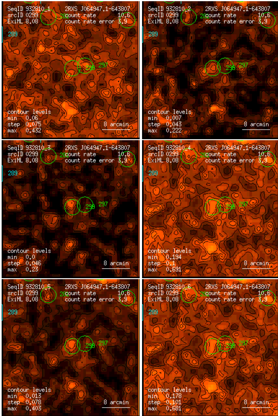
Figure 299: RASS 932810: detection 0299: band rate images, Gaussian filter: (1) PSPC channels 11 – 41, (2) 52 – 90, (3) 91 – 201, (4) 11 – 235, (5) 52 – 201, (6) 11 – 201. Broad band rates in counts/ks. Band rate contour levels in counts/ks/arcmin 2 .
