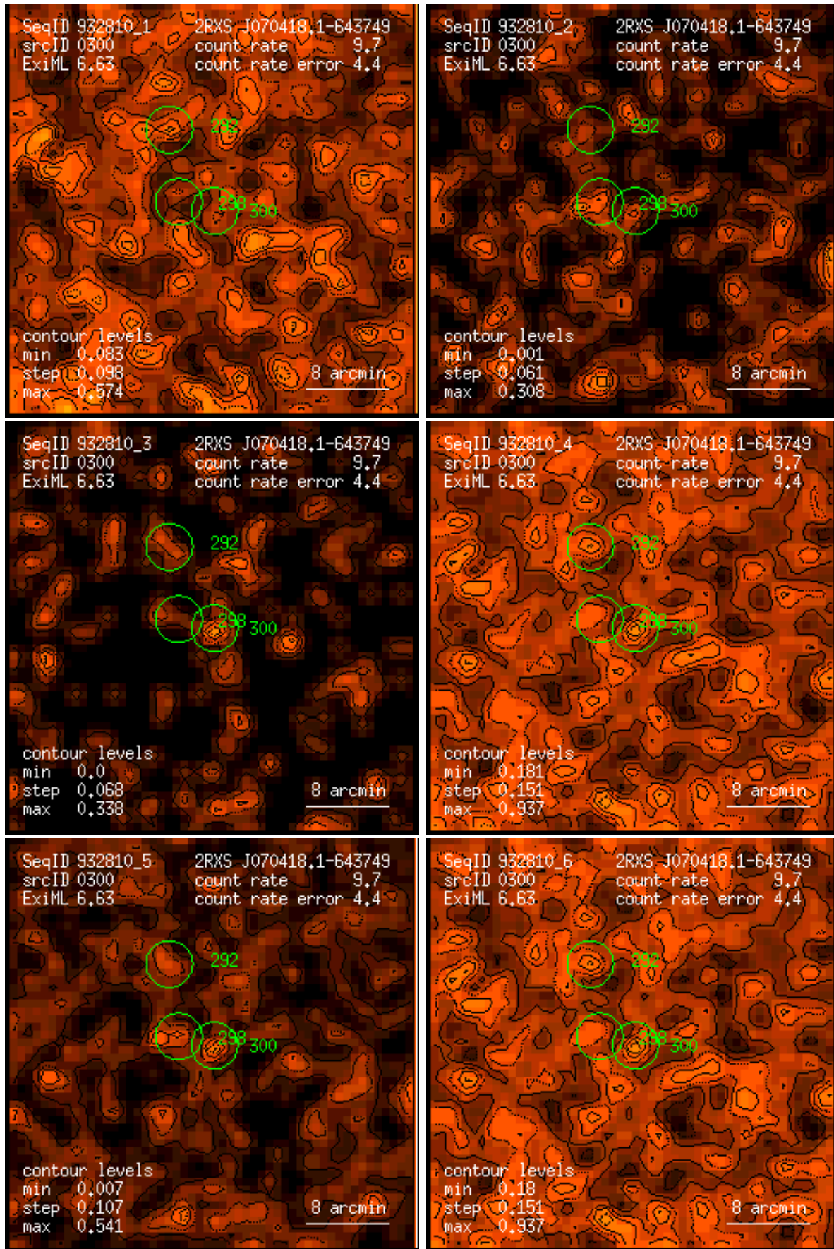
Figure 300: RASS 932810: detection 0300: band rate images, Gaussian filter: (1) PSPC channels 11 – 41, (2) 52 – 90, (3) 91 – 201, (4) 11 – 235, (5) 52 – 201, (6) 11 – 201. Broad band rates in counts/ks. Band rate contour levels in counts/ks/arcmin 2 .
