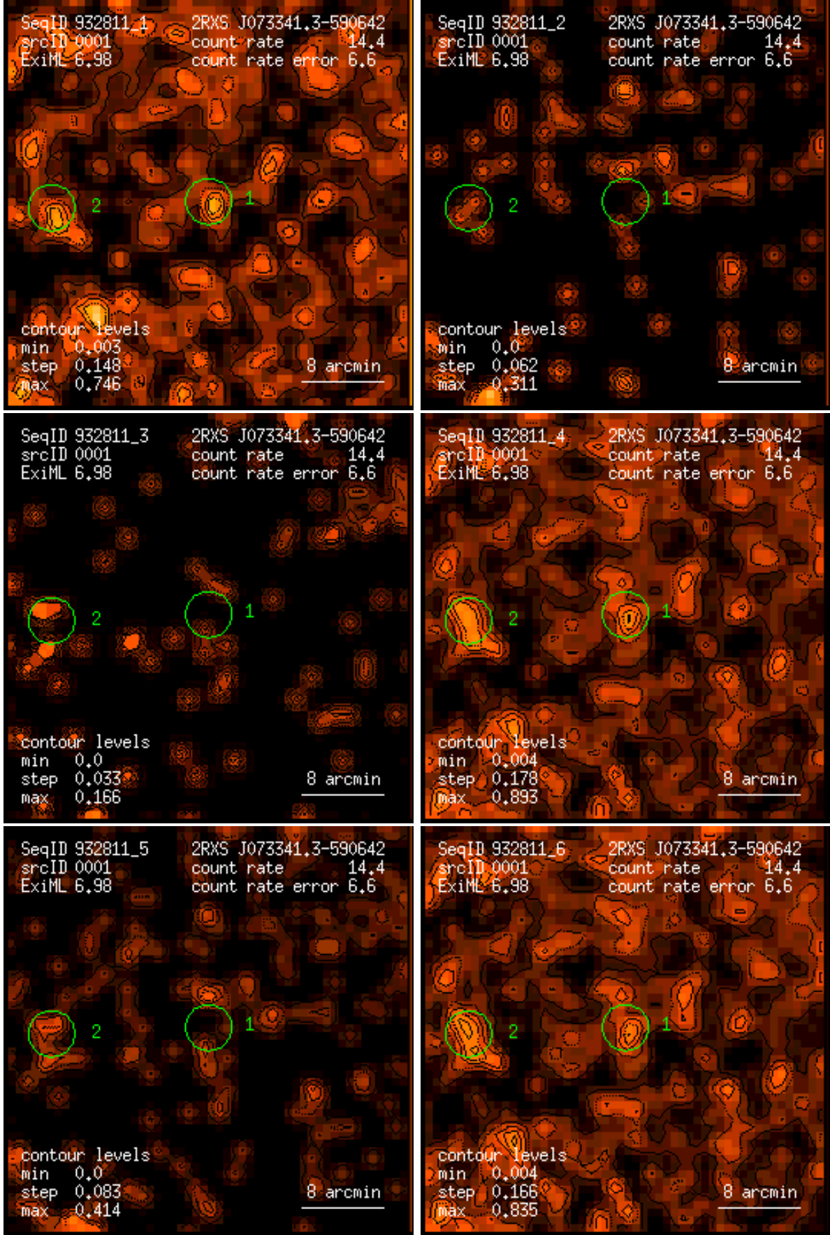
Figure 1: RASS 932811: detection 0001: band rate images, Gaussian filter: (1) PSPC channels 11 – 41, (2) 52 – 90, (3) 91 – 201, (4) 11 – 235, (5) 52 – 201, (6) 11 – 201. Broad band rates in counts/ks. Band rate contour levels in counts/ks/arcmin 2 .
