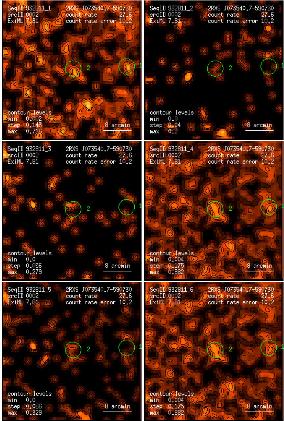
Figure 2: RASS 932811: detection 0002: band rate images, Gaussian filter: (1) PSPC channels 11 – 41, (2) 52 – 90, (3) 91 – 201, (4) 11 – 235, (5) 52 – 201, (6) 11 – 201. Broad band rates in counts/ks. Band rate contour levels in counts/ks/arcmin 2 .
