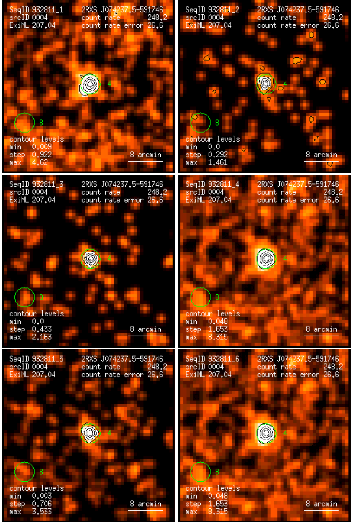
Figure 4: RASS 932811: detection 0004: band rate images, Gaussian filter: (1) PSPC channels 11 – 41, (2) 52 – 90, (3) 91 – 201, (4) 11 – 235, (5) 52 – 201, (6) 11 – 201. Broad band rates in counts/ks. Band rate contour levels in counts/ks/arcmin 2 .
