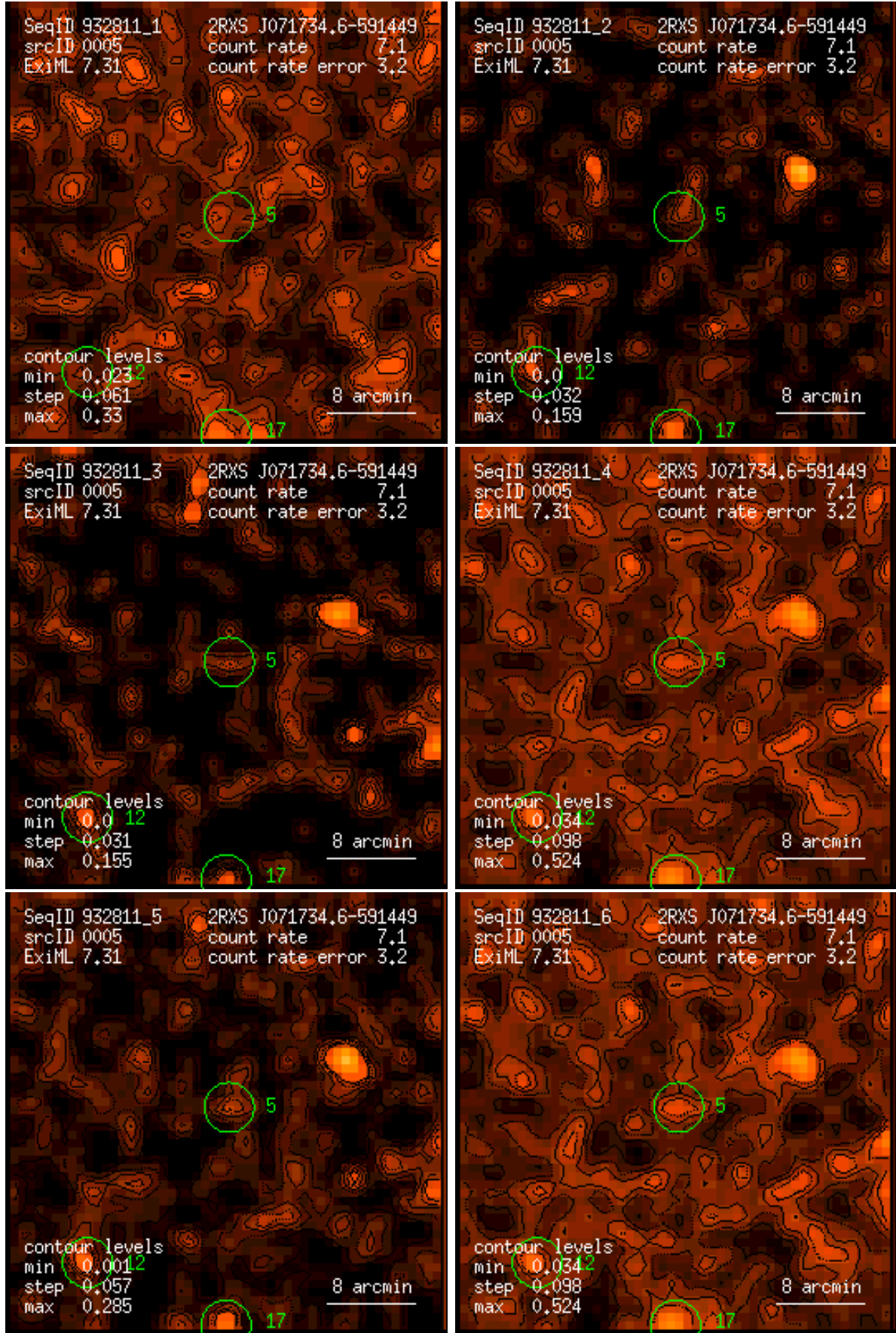
Figure 5: RASS 932811: detection 0005: band rate images, Gaussian filter: (1) PSPC channels 11 – 41, (2) 52 – 90, (3) 91 – 201, (4) 11 – 235, (5) 52 – 201, (6) 11 – 201. Broad band rates in counts/ks. Band rate contour levels in counts/ks/arcmin 2 .
