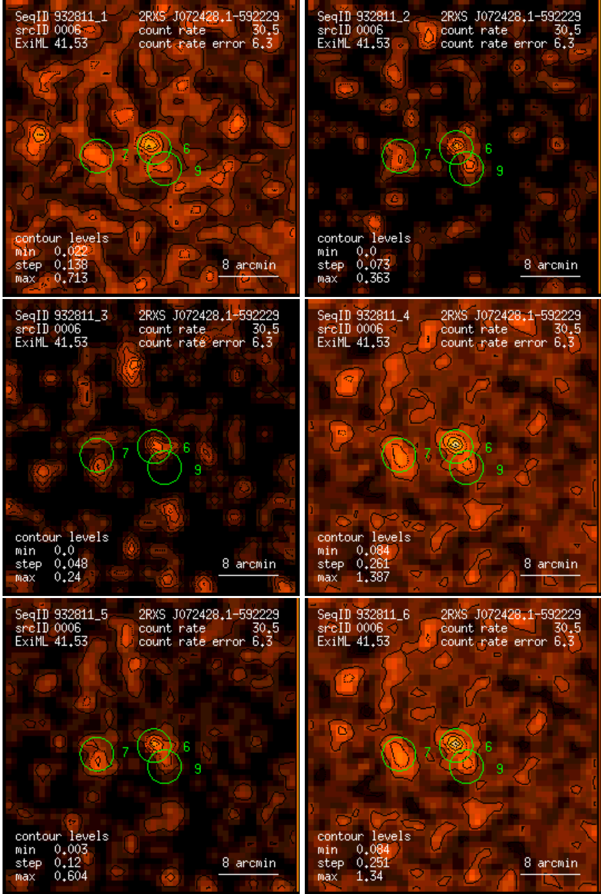
Figure 6: RASS 932811: detection 0006: band rate images, Gaussian filter: (1) PSPC channels 11 – 41, (2) 52 – 90, (3) 91 – 201, (4) 11 – 235, (5) 52 – 201, (6) 11 – 201. Broad band rates in counts/ks. Band rate contour levels in counts/ks/arcmin 2 .
