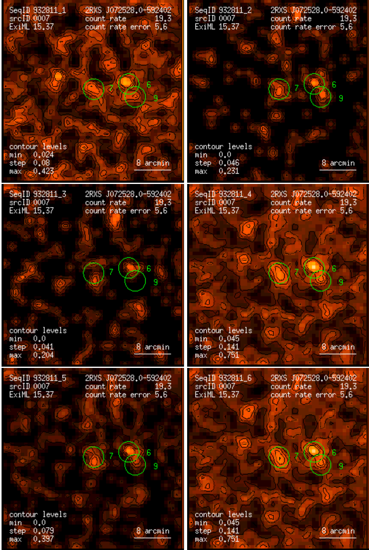
Figure 7: RASS 932811: detection 0007: band rate images, Gaussian filter: (1) PSPC channels 11 – 41, (2) 52 – 90, (3) 91 – 201, (4) 11 – 235, (5) 52 – 201, (6) 11 – 201. Broad band rates in counts/ks. Band rate contour levels in counts/ks/arcmin 2 .
