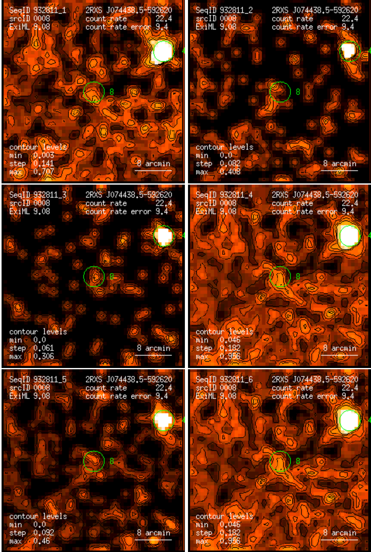
Figure 8: RASS 932811: detection 0008: band rate images, Gaussian filter: (1) PSPC channels 11 – 41, (2) 52 – 90, (3) 91 – 201, (4) 11 – 235, (5) 52 – 201, (6) 11 – 201. Broad band rates in counts/ks. Band rate contour levels in counts/ks/arcmin 2 .
