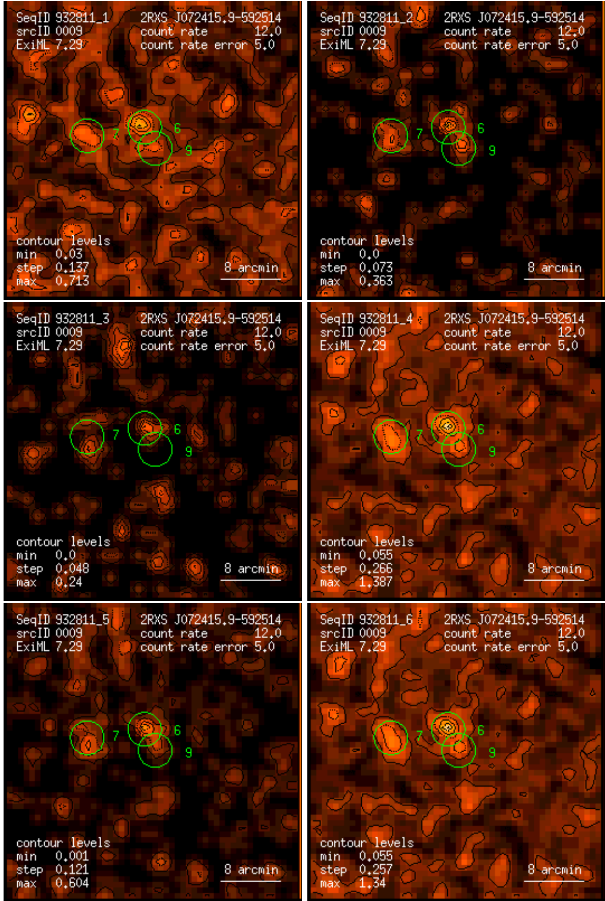
Figure 9: RASS 932811: detection 0009: band rate images, Gaussian filter: (1) PSPC channels 11 – 41, (2) 52 – 90, (3) 91 – 201, (4) 11 – 235, (5) 52 – 201, (6) 11 – 201. Broad band rates in counts/ks. Band rate contour levels in counts/ks/arcmin 2 .
