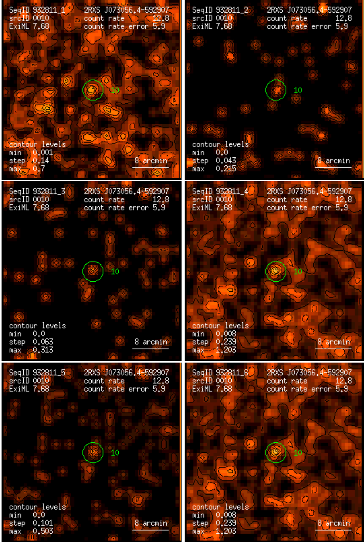
Figure 10: RASS 932811: detection 0010: band rate images, Gaussian filter: (1) PSPC channels 11 – 41, (2) 52 – 90, (3) 91 – 201, (4) 11 – 235, (5) 52 – 201, (6) 11 – 201. Broad band rates in counts/ks. Band rate contour levels in counts/ks/arcmin 2 .
