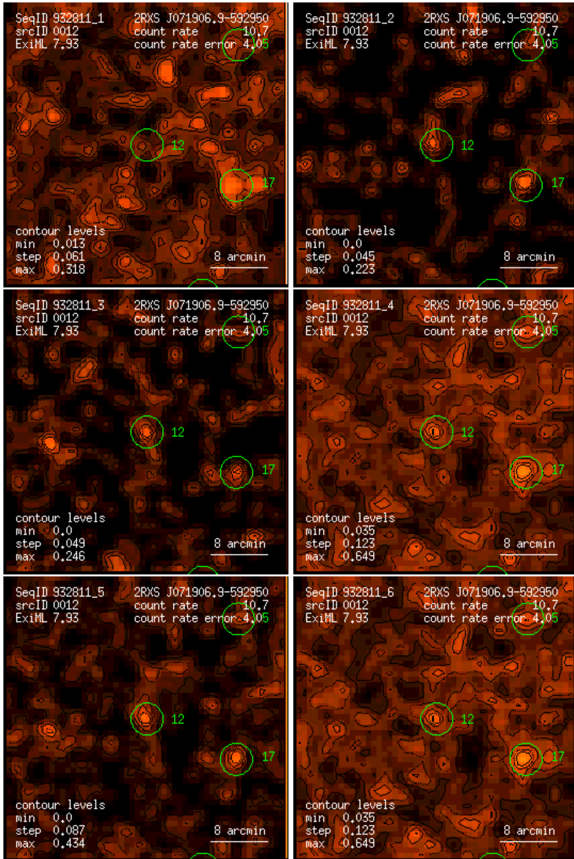
Figure 12: RASS 932811: detection 0012: band rate images, Gaussian filter: (1) PSPC channels 11 – 41, (2) 52 – 90, (3) 91 – 201, (4) 11 – 235, (5) 52 – 201, (6) 11 – 201. Broad band rates in counts/ks. Band rate contour levels in counts/ks/arcmin 2 .
