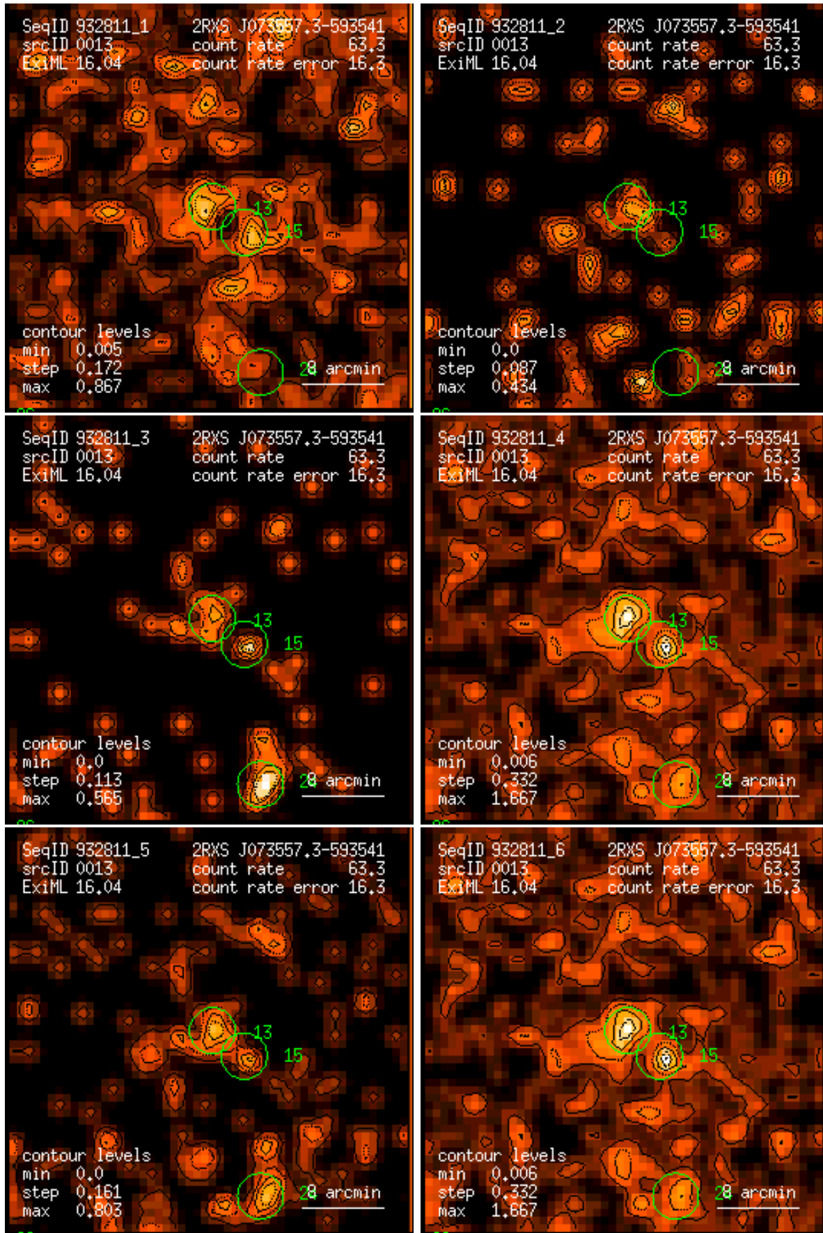
Figure 13: RASS 932811: detection 0013: band rate images, Gaussian filter: (1) PSPC channels 11 – 41, (2) 52 – 90, (3) 91 – 201, (4) 11 – 235, (5) 52 – 201, (6) 11 – 201. Broad band rates in counts/ks. Band rate contour levels in counts/ks/arcmin 2 .
