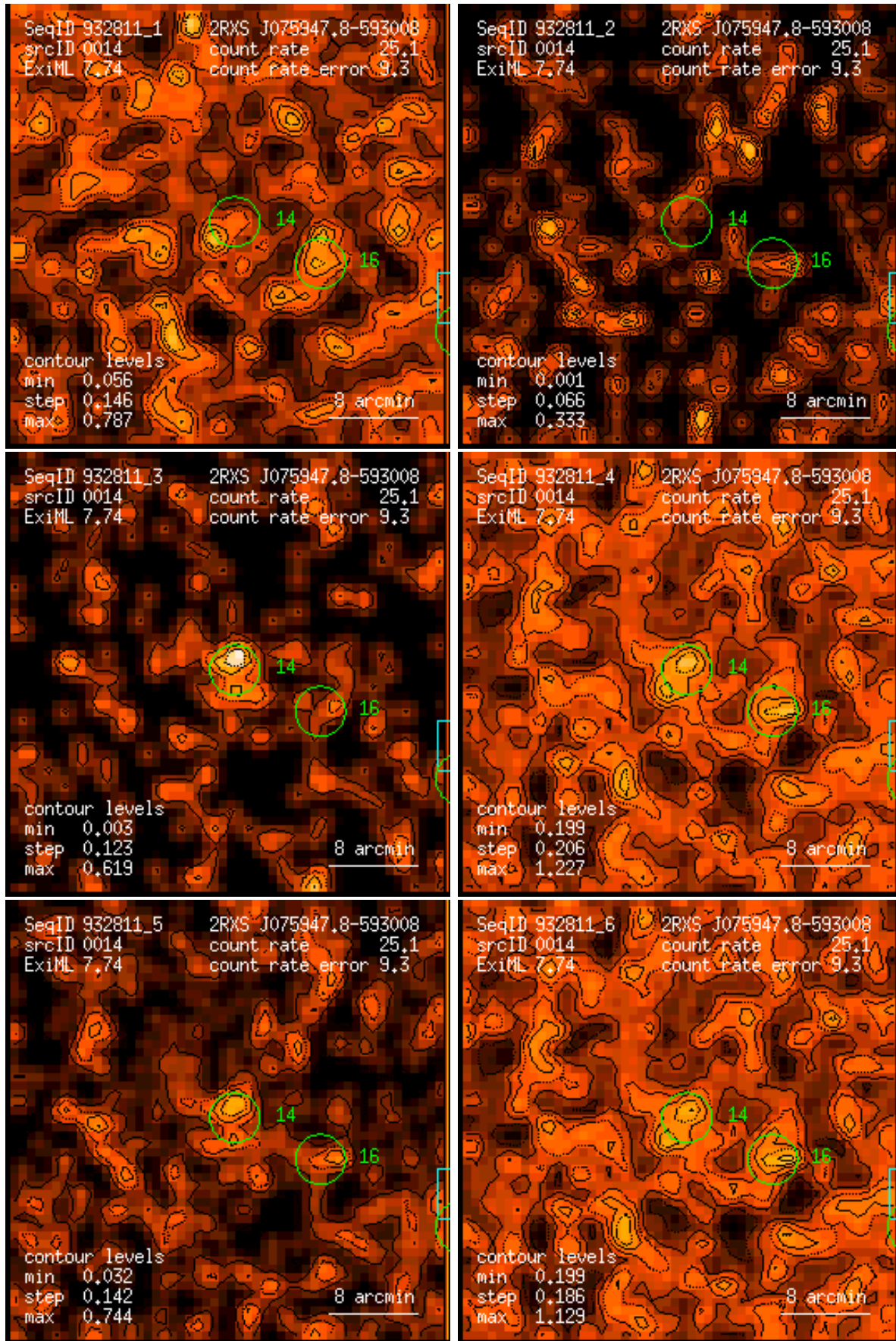
Figure 14: RASS 932811: detection 0014: band rate images, Gaussian filter: (1) PSPC channels 11 – 41, (2) 52 – 90, (3) 91 – 201, (4) 11 – 235, (5) 52 – 201, (6) 11 – 201. Broad band rates in counts/ks. Band rate contour levels in counts/ks/arcmin 2 .
